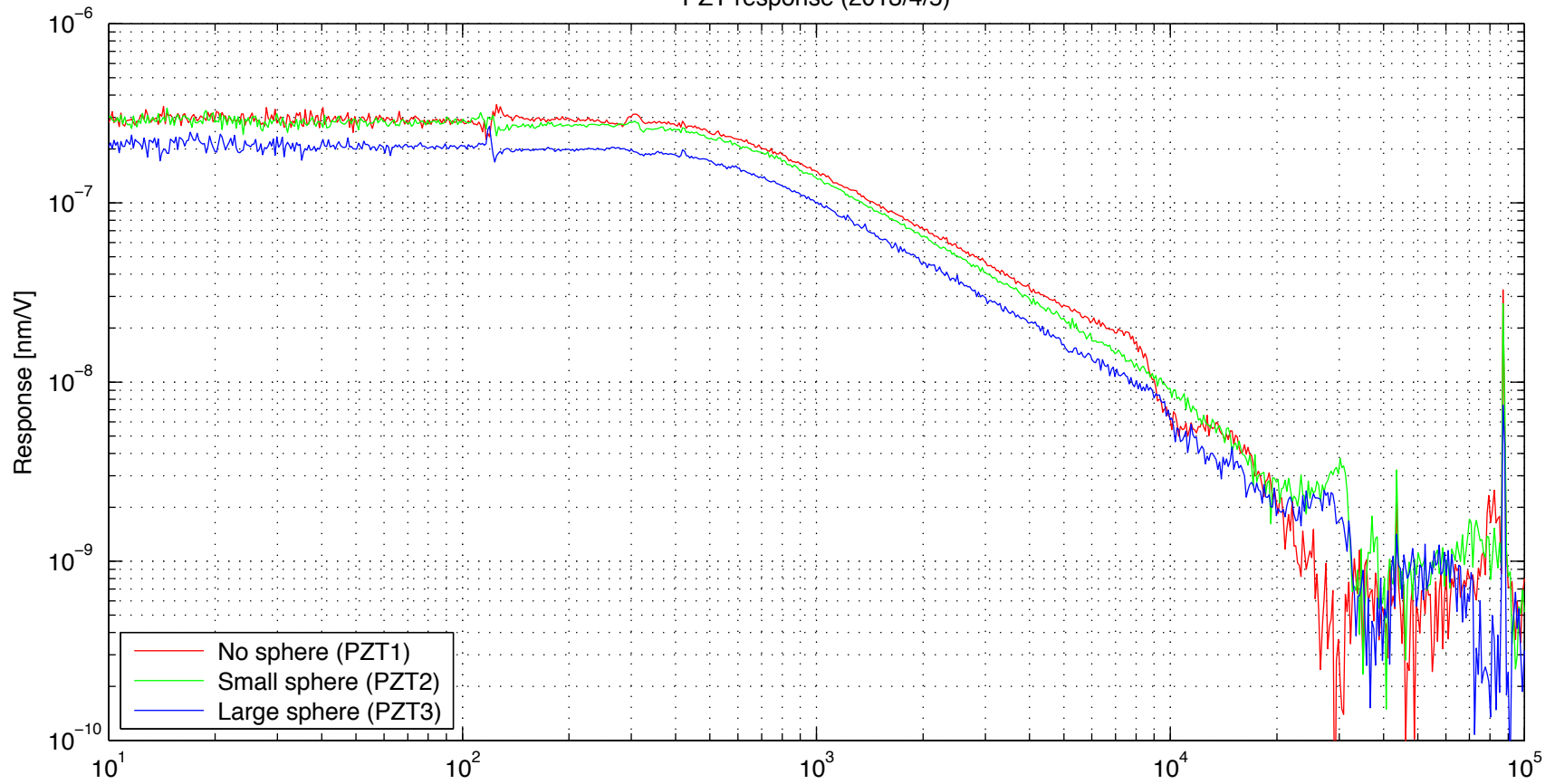
PZT response (2013/4/5)
