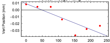
Vertical Wedge Fitting ~ A1
