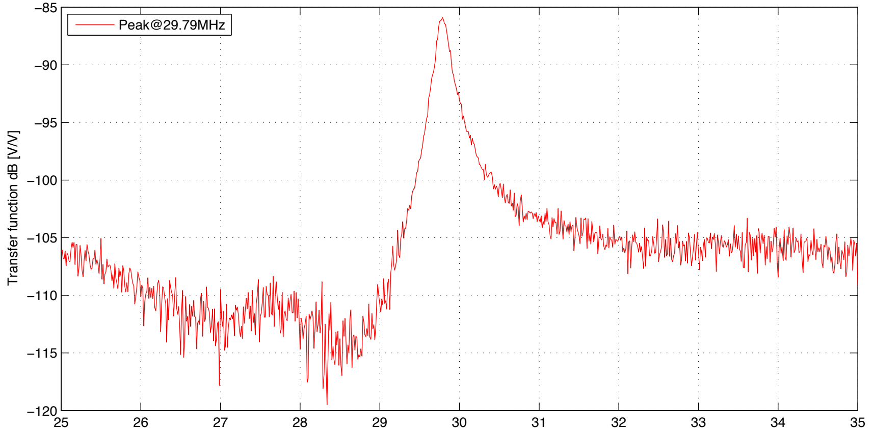
RoC measurement (2012/10/16)
