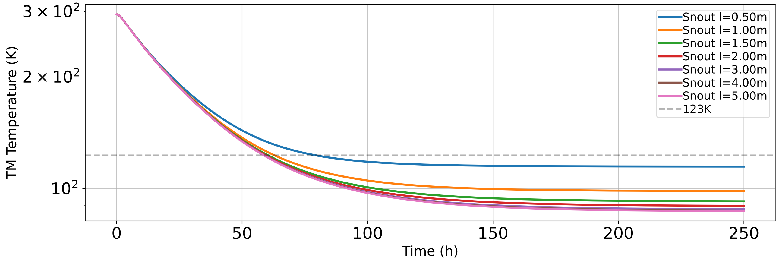
Mariner ITM: Radiative Cooldown
