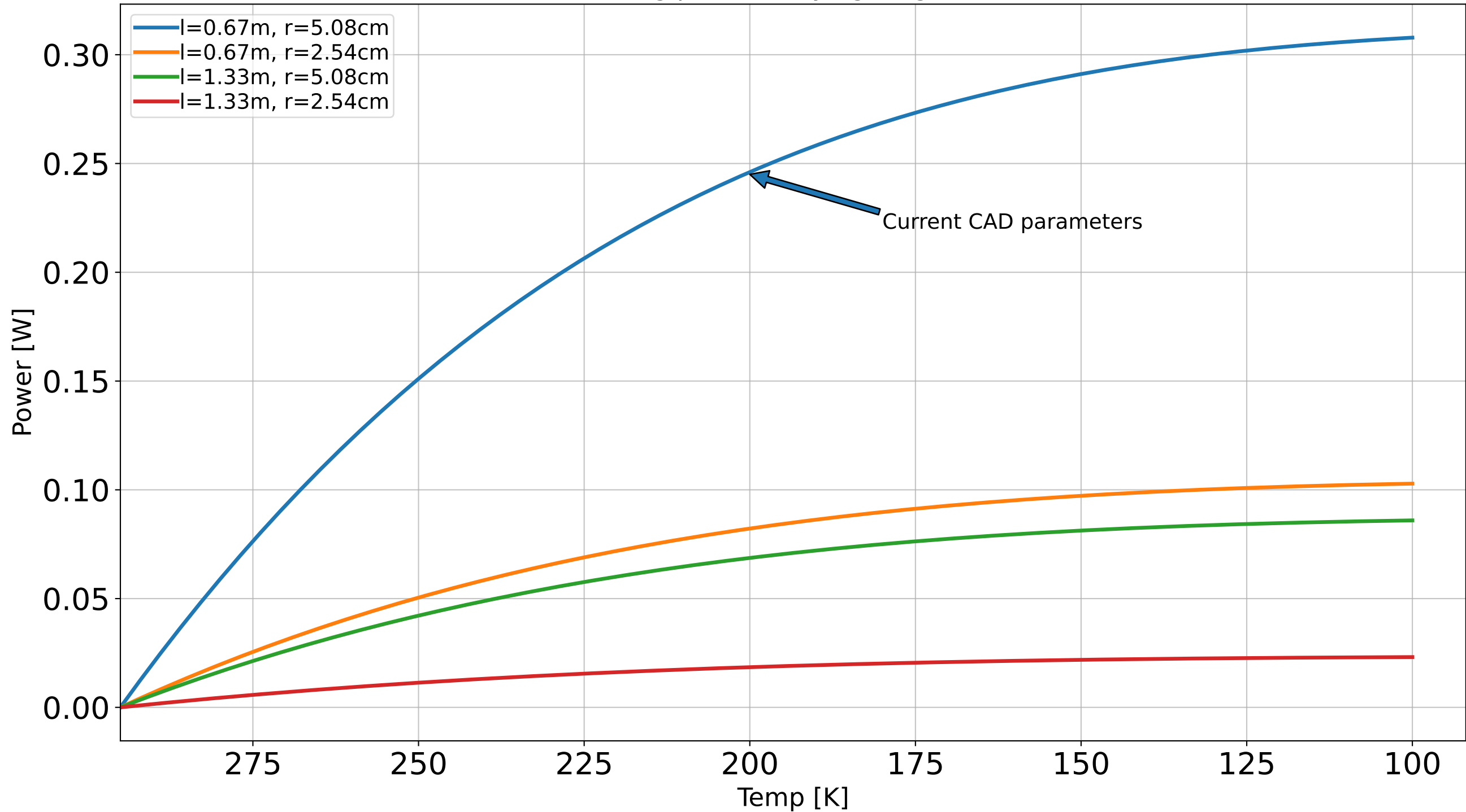
Snout heating power, varying length and radius
