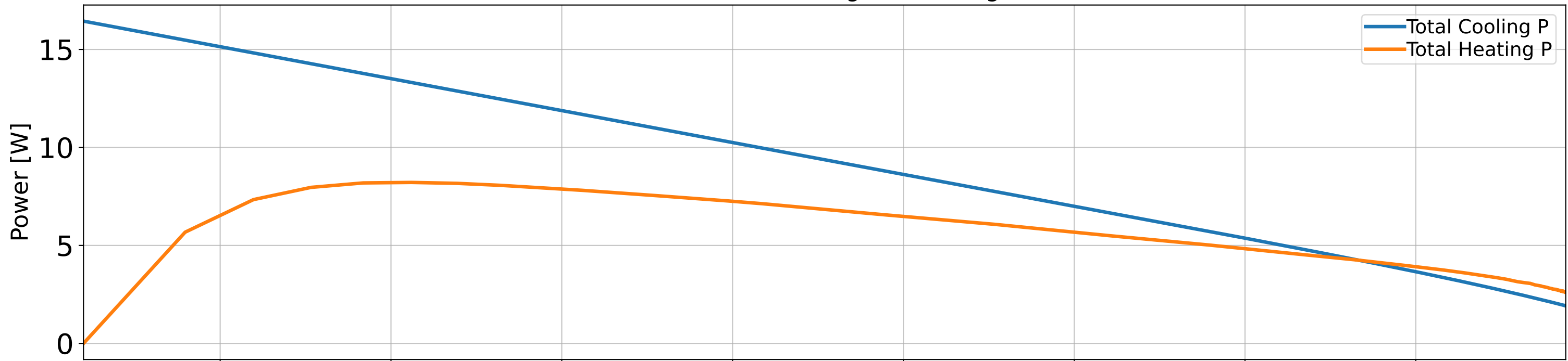
Inner shield Cooling vs. Heating P
