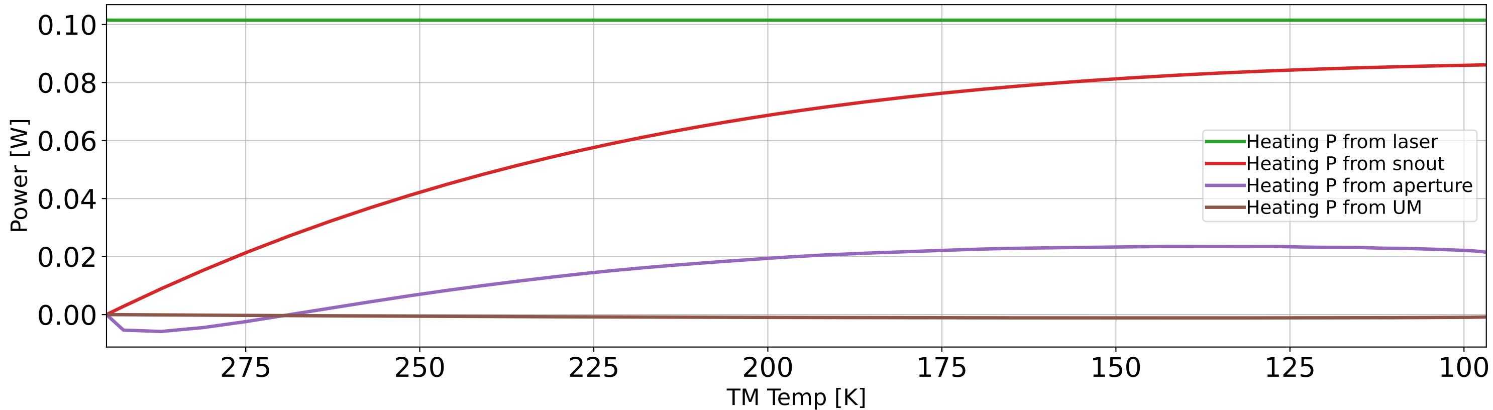
Heat loads
