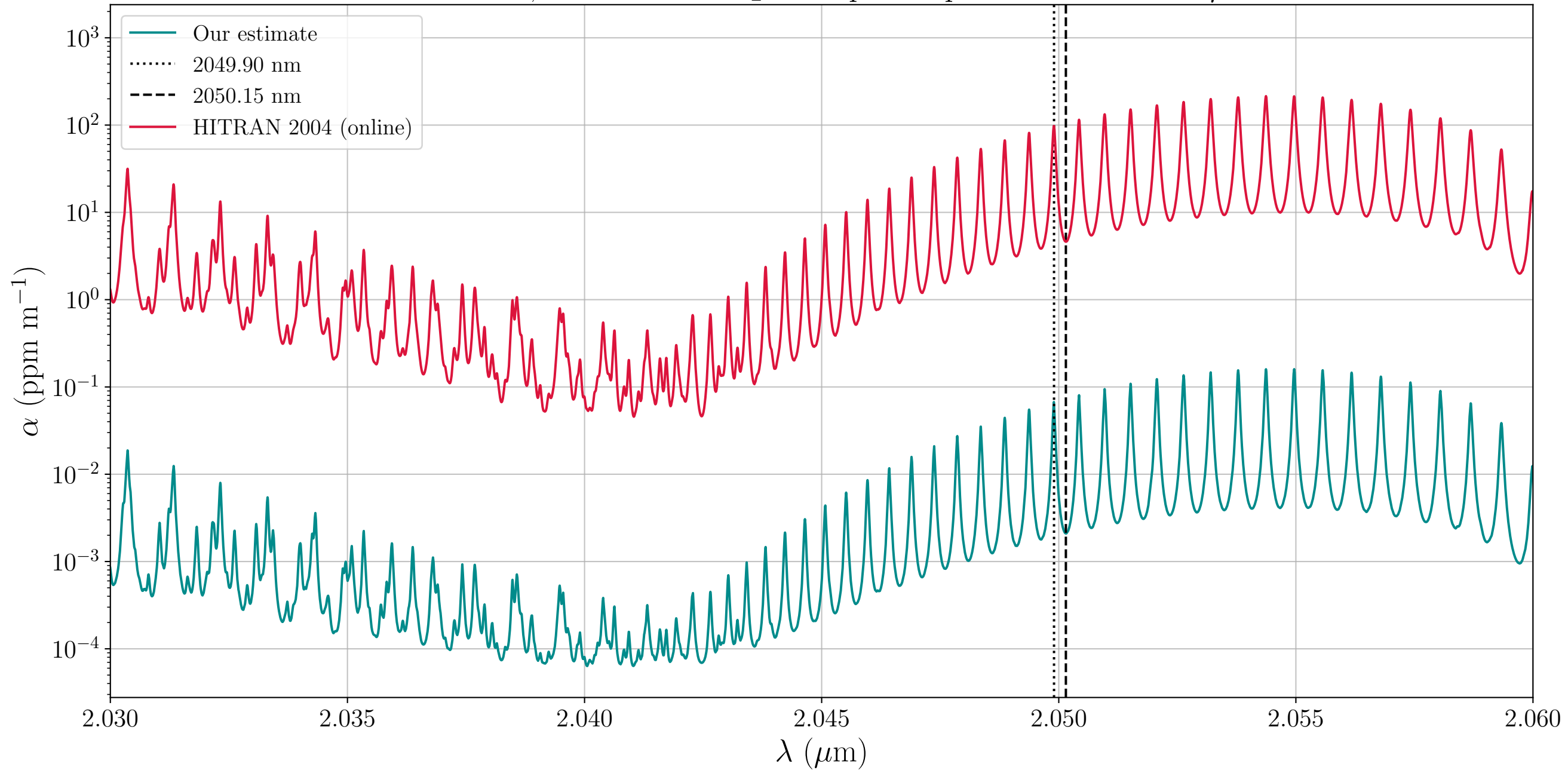
P = 1 atm, T = 296 K \text{CO}_2 absorption spectrum near 2.05 \mu\text{m}
