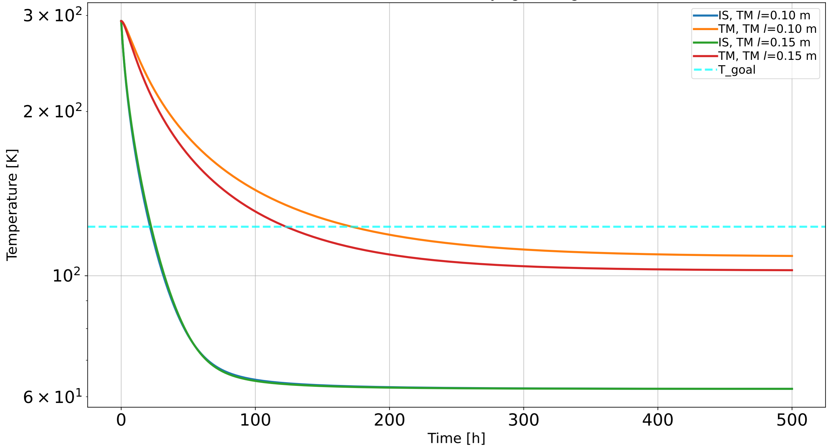
Test mass cooldown, varying TM length
