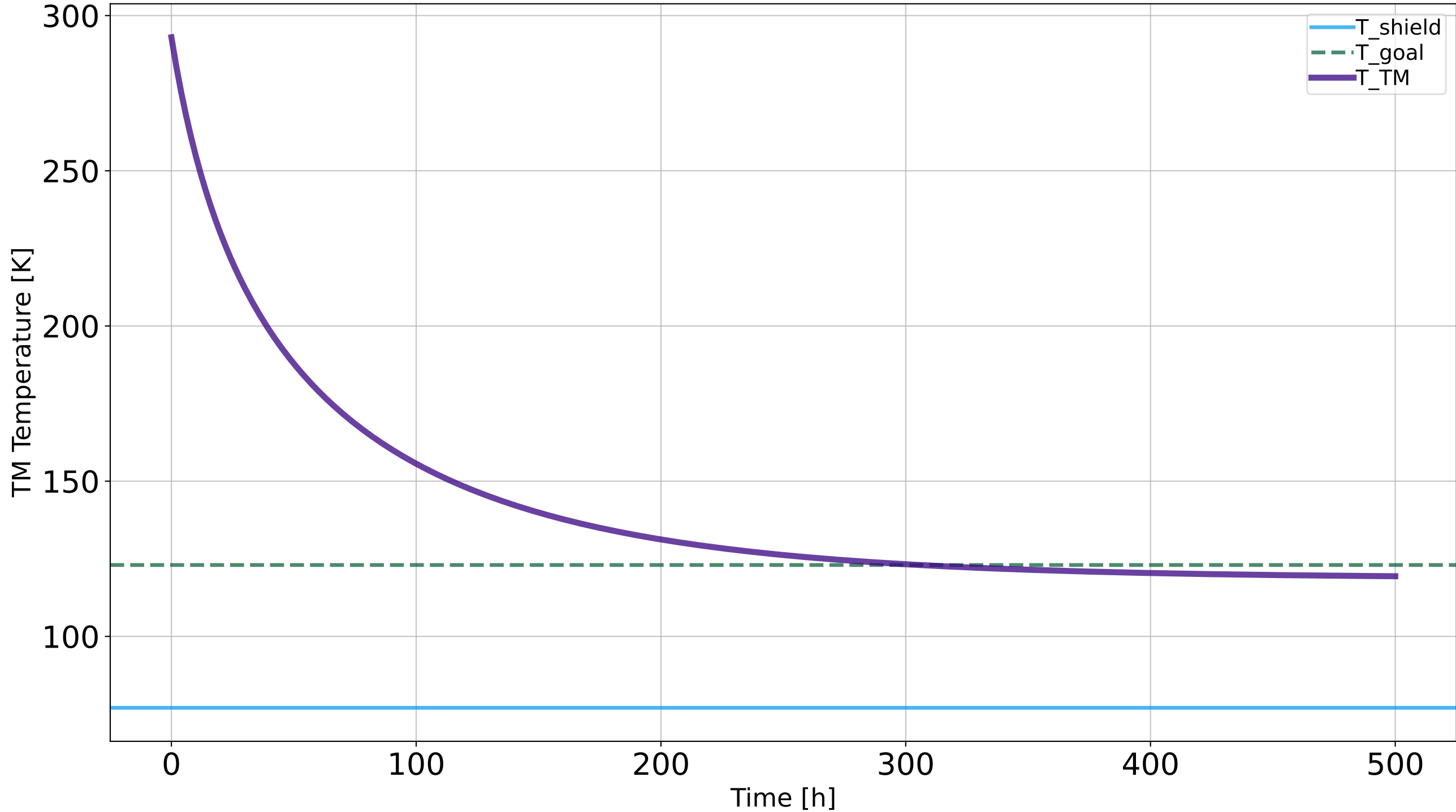
Mariner ITM: Radiative Cooledown
