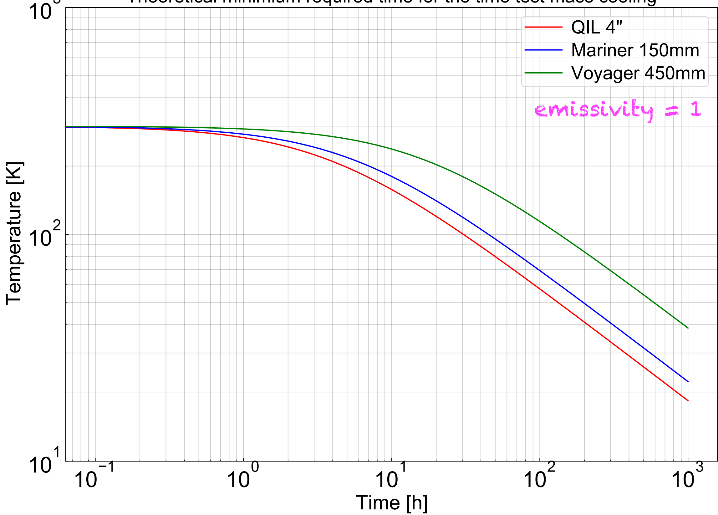
Theoretical minimum required time for the time test mass cooling
