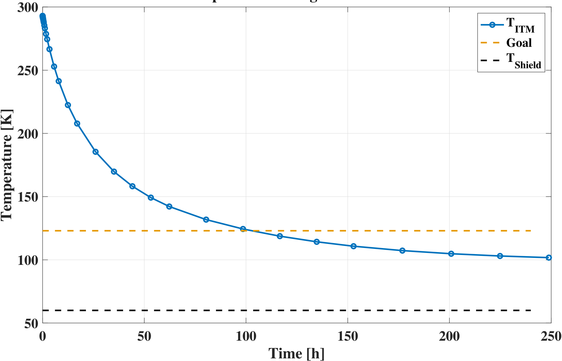
ITM Temperature during radiative cooldown
