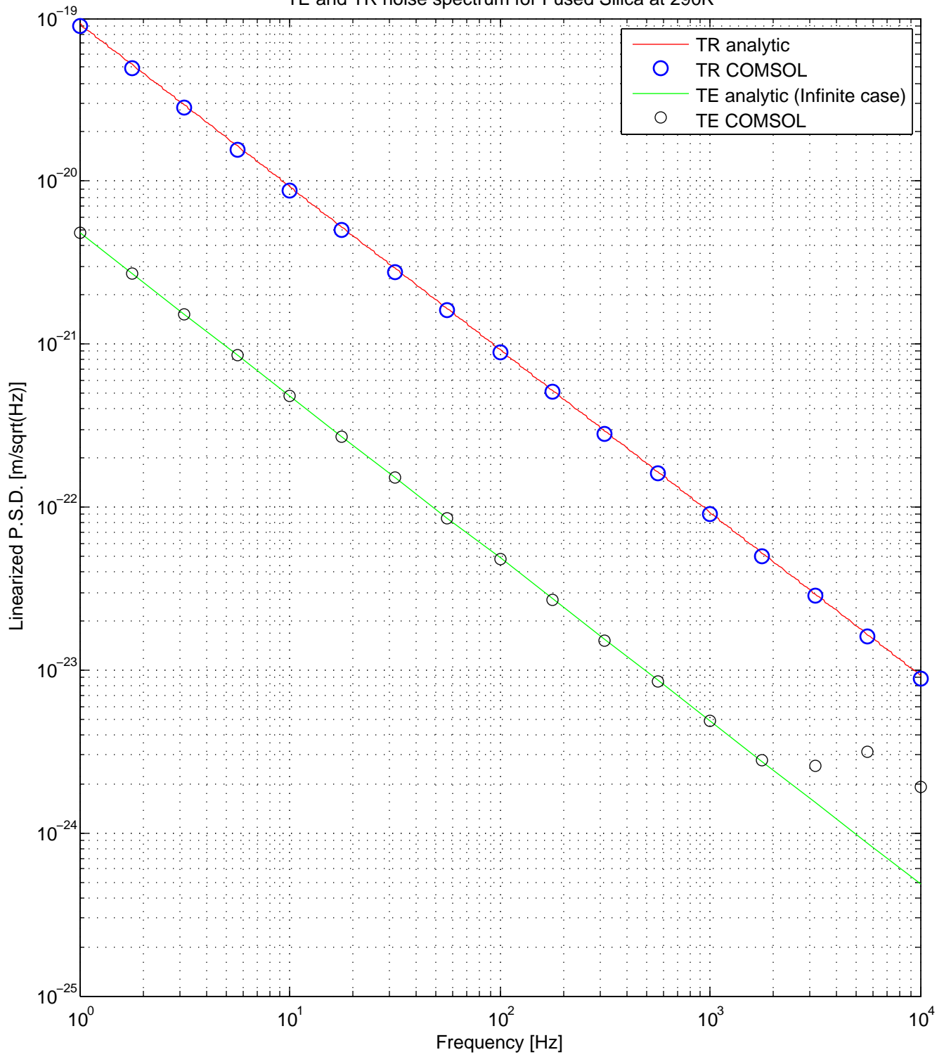
TE and TR noise spectrum for Fused Silica at 290K
