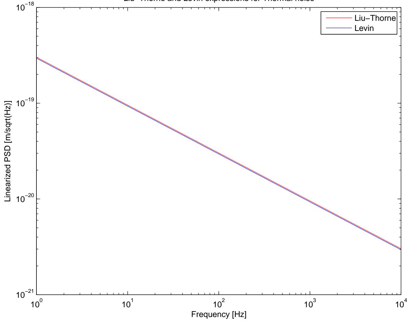
Liu-Thorne and Levin expressions for Thermal noise
