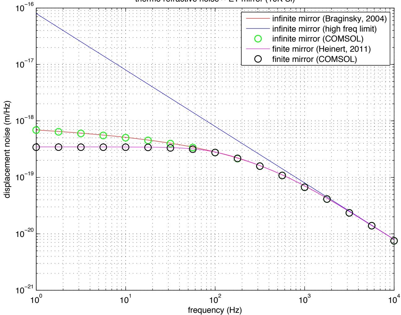
thermo refractive noise ~ ET mirror (10K Si)
