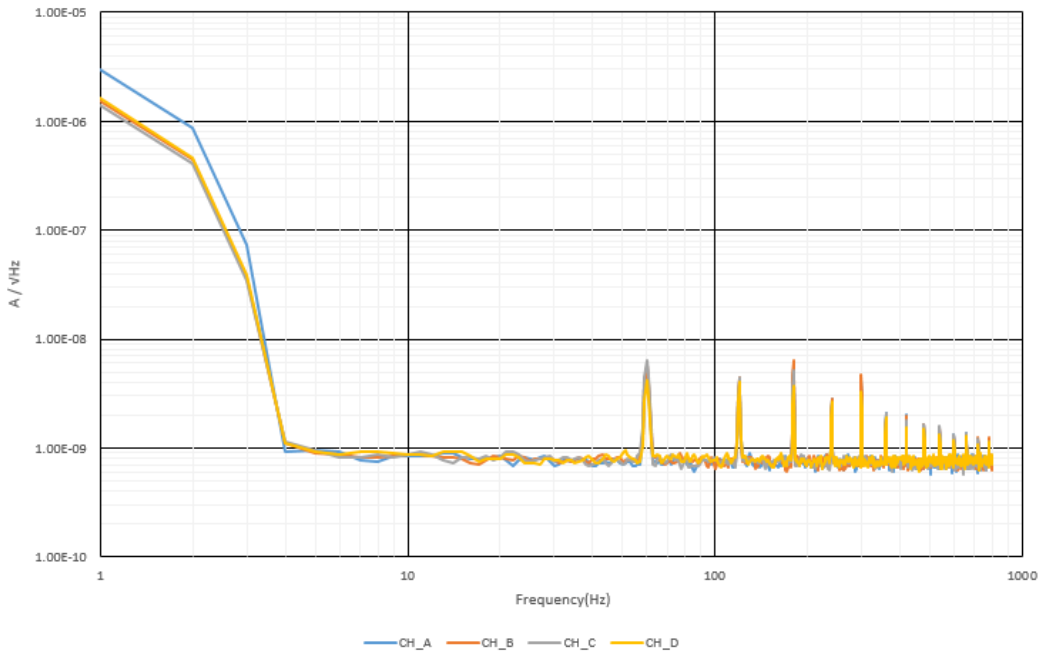
LED Current Supply Noise D1900217 S1900540
