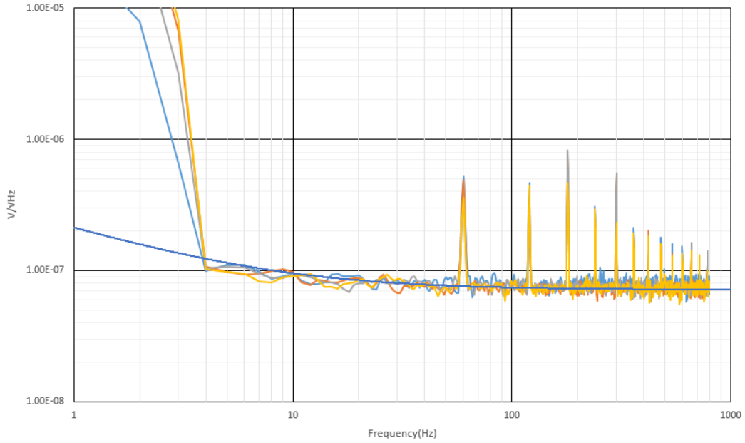
LED Voltage Noise at R48(100Ω) D1900217 S1900541
