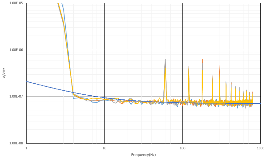
LED Voltage Noise at R48(100Ω) D1900217 S1900540
