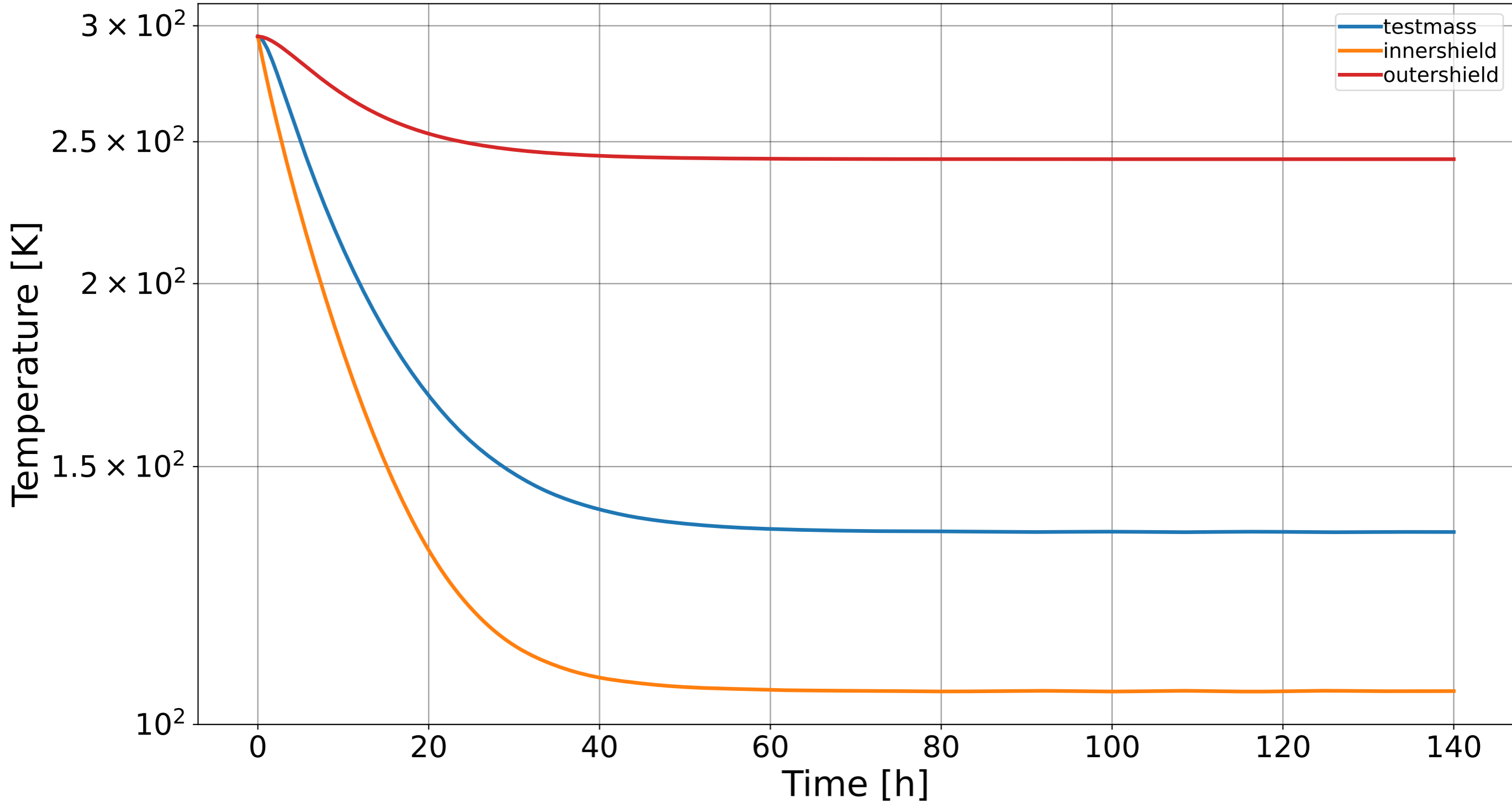
PSOMAstat Cooldown Model
