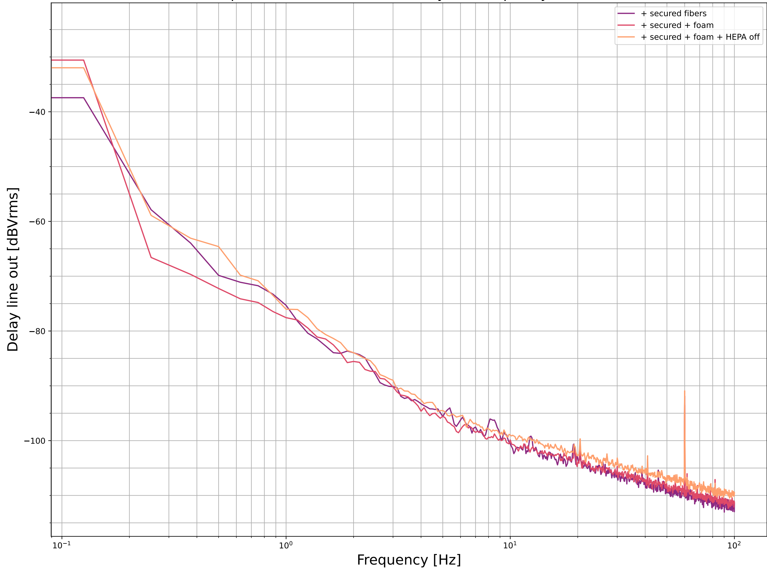
SR785 spectrum of Rio E x Rio W delay line frequency discriminator
