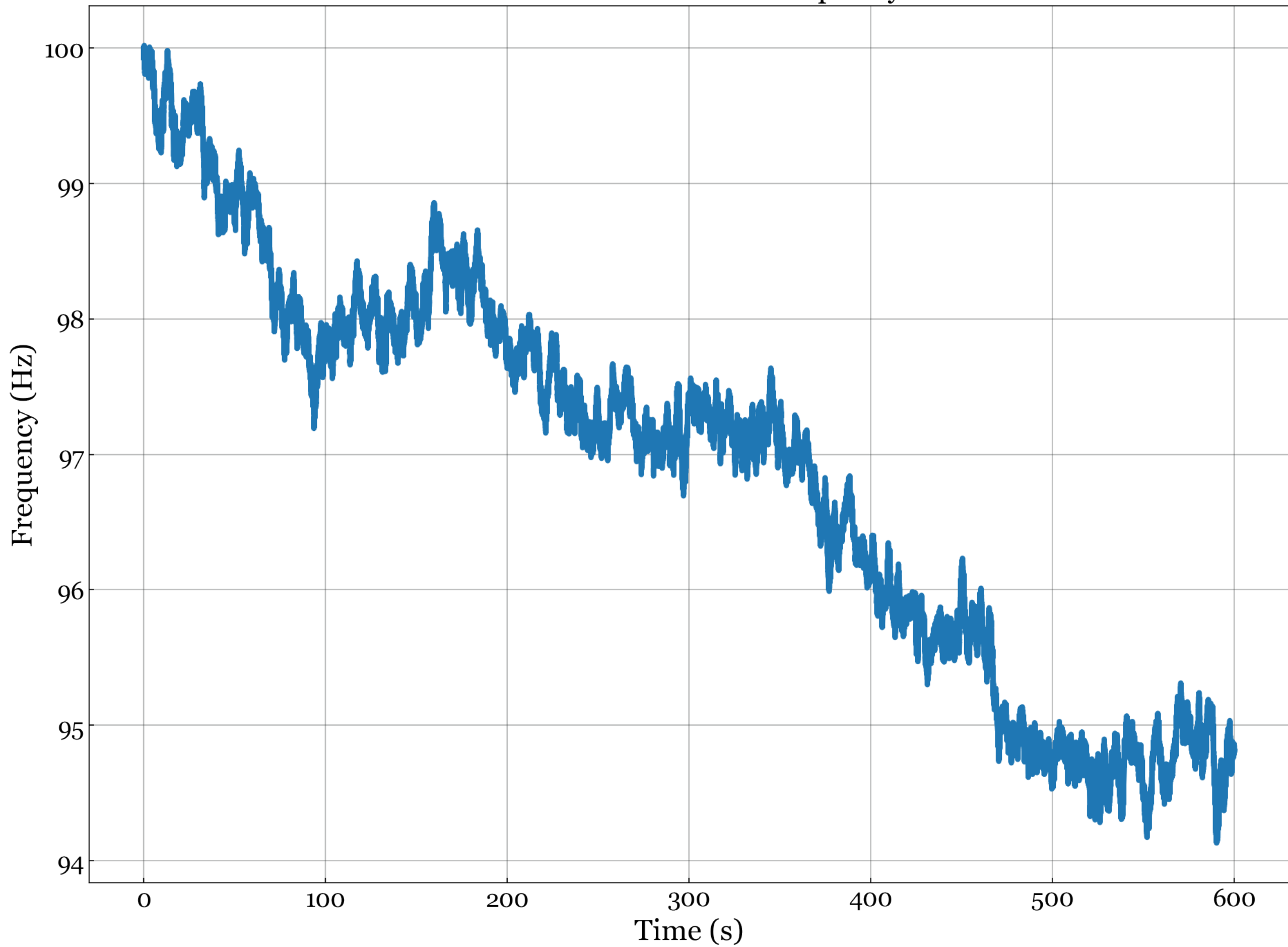
Rio W x Teraxion beat frequency
