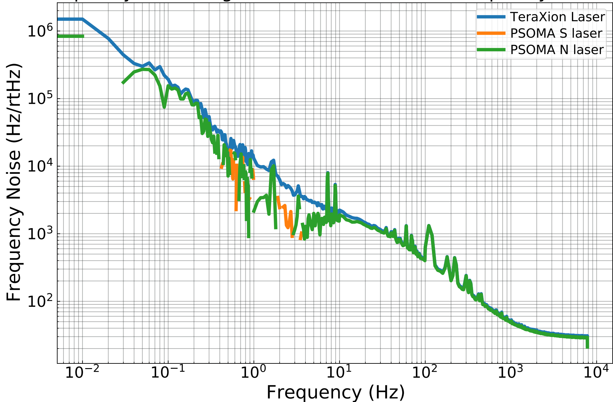
Frequency ASD using Three Corner Hat, from frequency estimate
