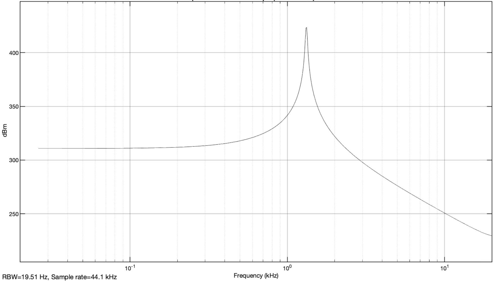
Power Spectrum of Excited Sample (mode f=1038)
