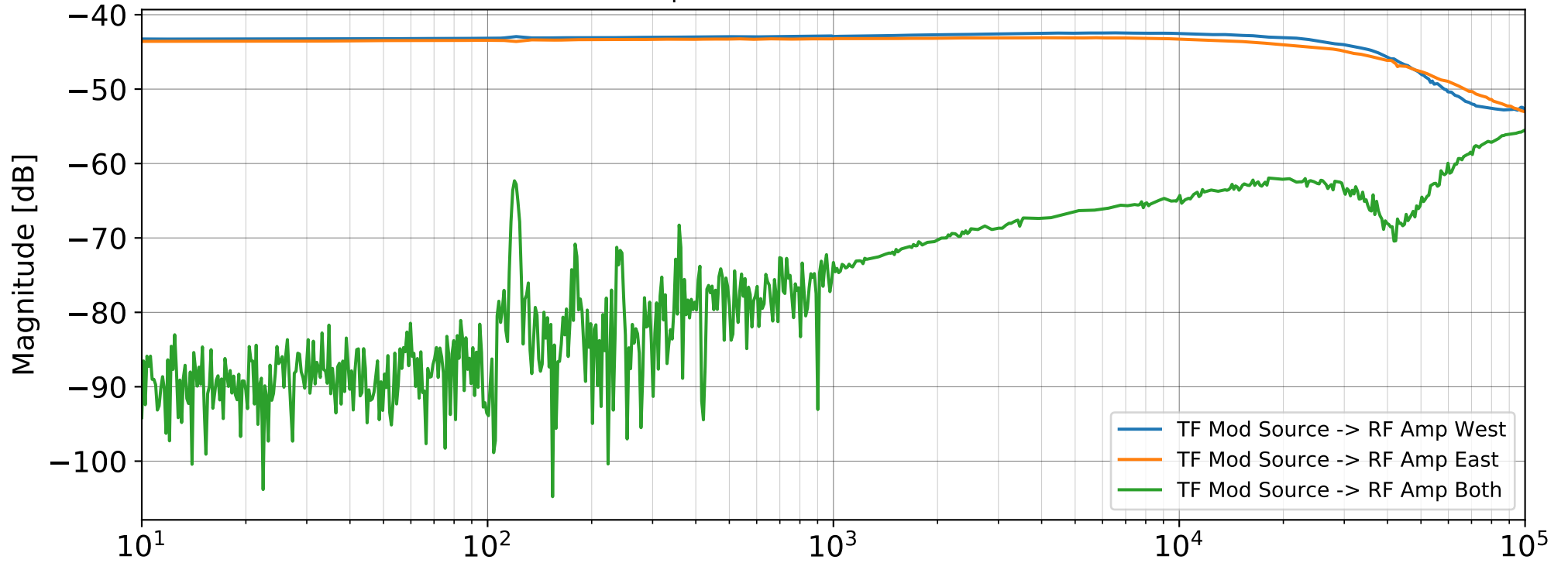
Beat Amplitude Modulation AOM 20180623
