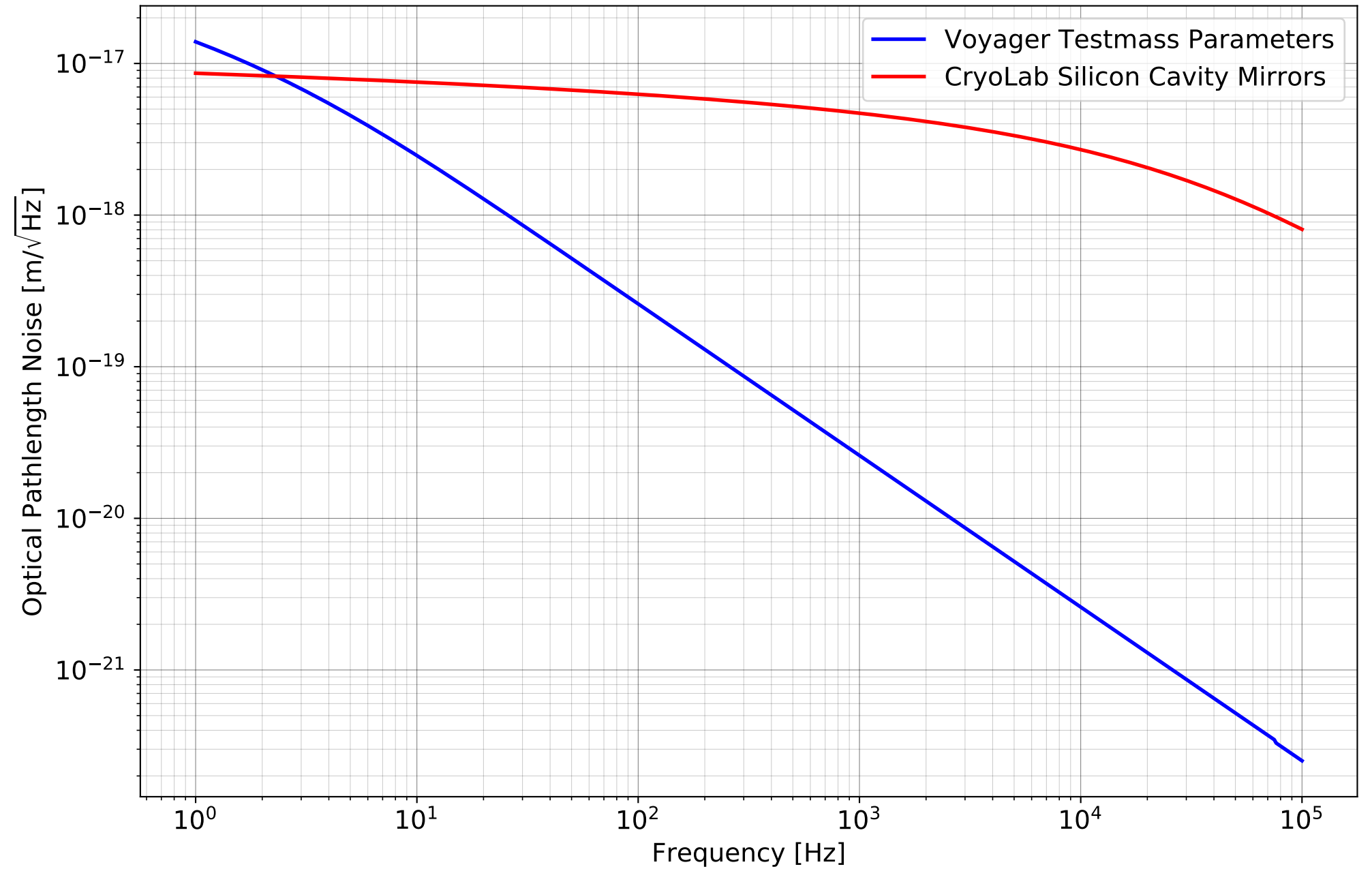
Single Pass Substrate Carrier Density Noise Optical Pathlength Noise
