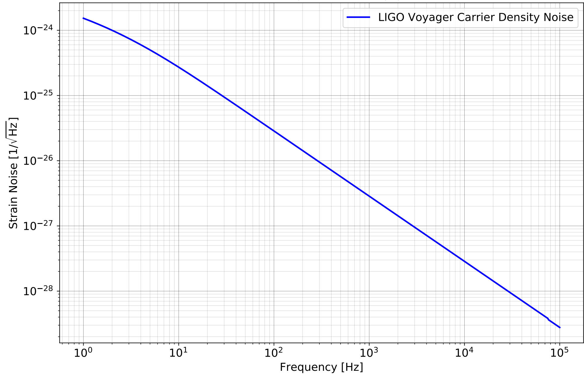
Carrier Density Noise in LIGO Voyager
