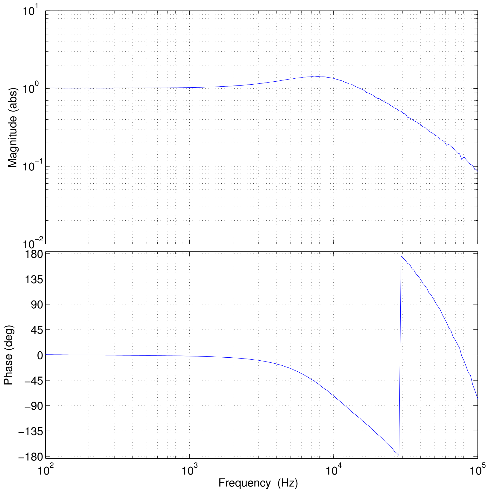
Bode Diagram
