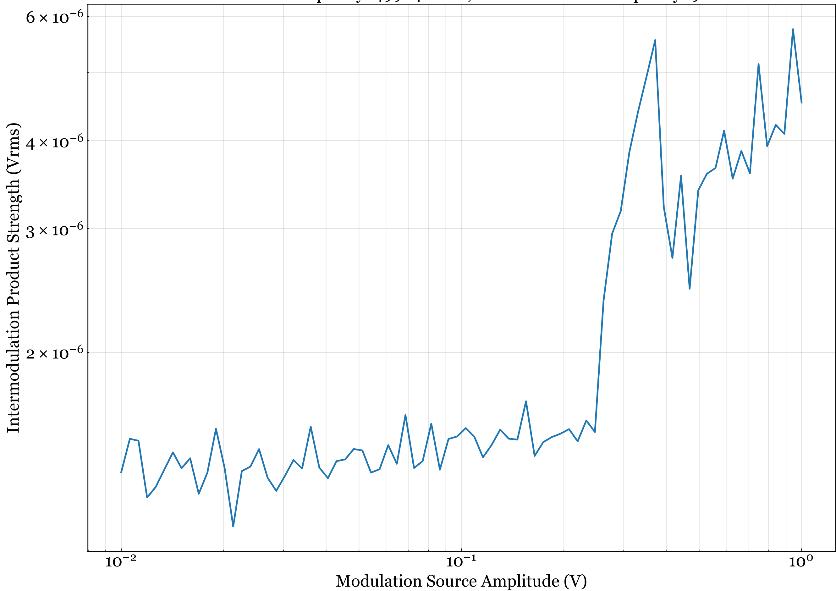
SR785 Self IP2 measurement Modulation Frequency: 49984 Hz ; Intermodulation Frequency: 96Hz
