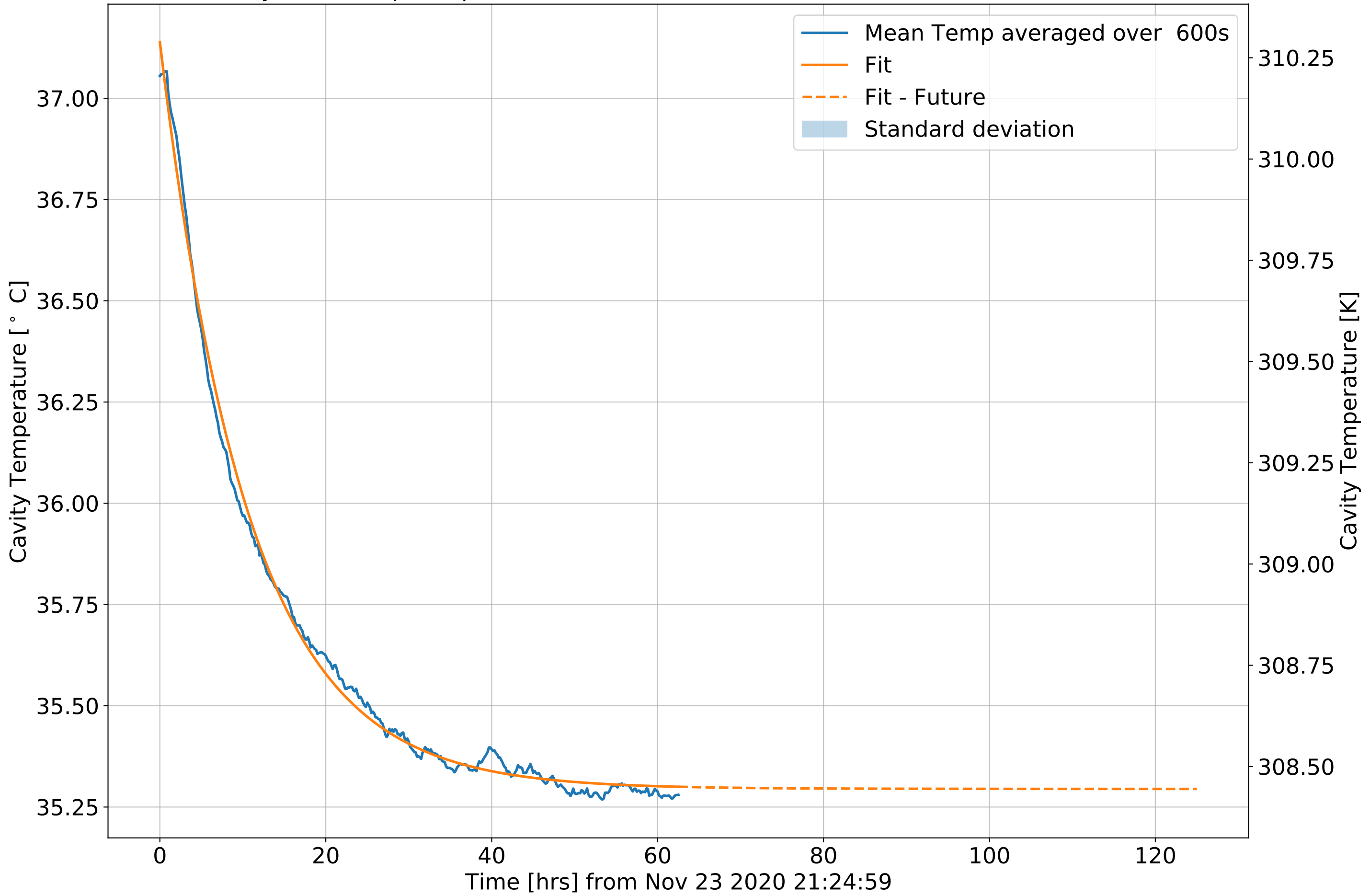
Cavity Out-of-loop Temperature from Nov 23 2020 21:24:59 to Nov 26 2020 11:54:59
