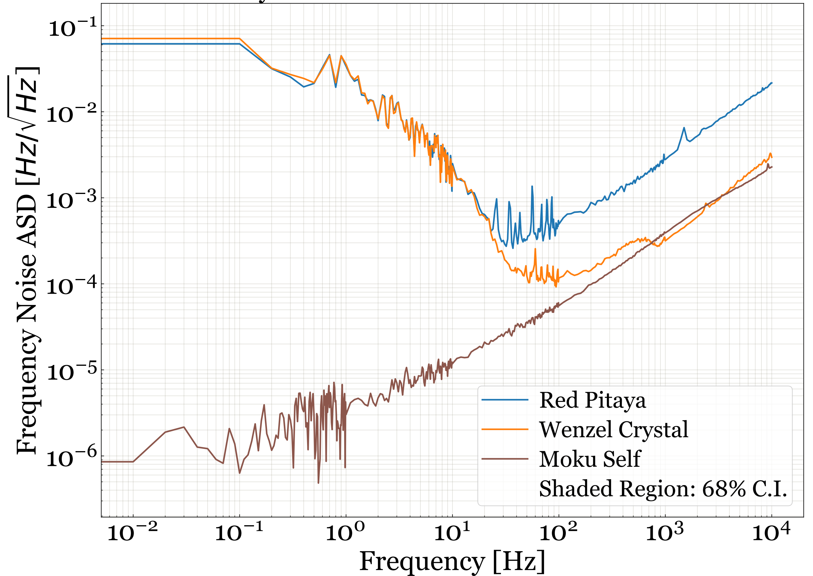
Comparison of Red Pitaya and Wenzel Crystal frequency noise measured by Moku Phasemeter with 10 kHz Bandwidth
