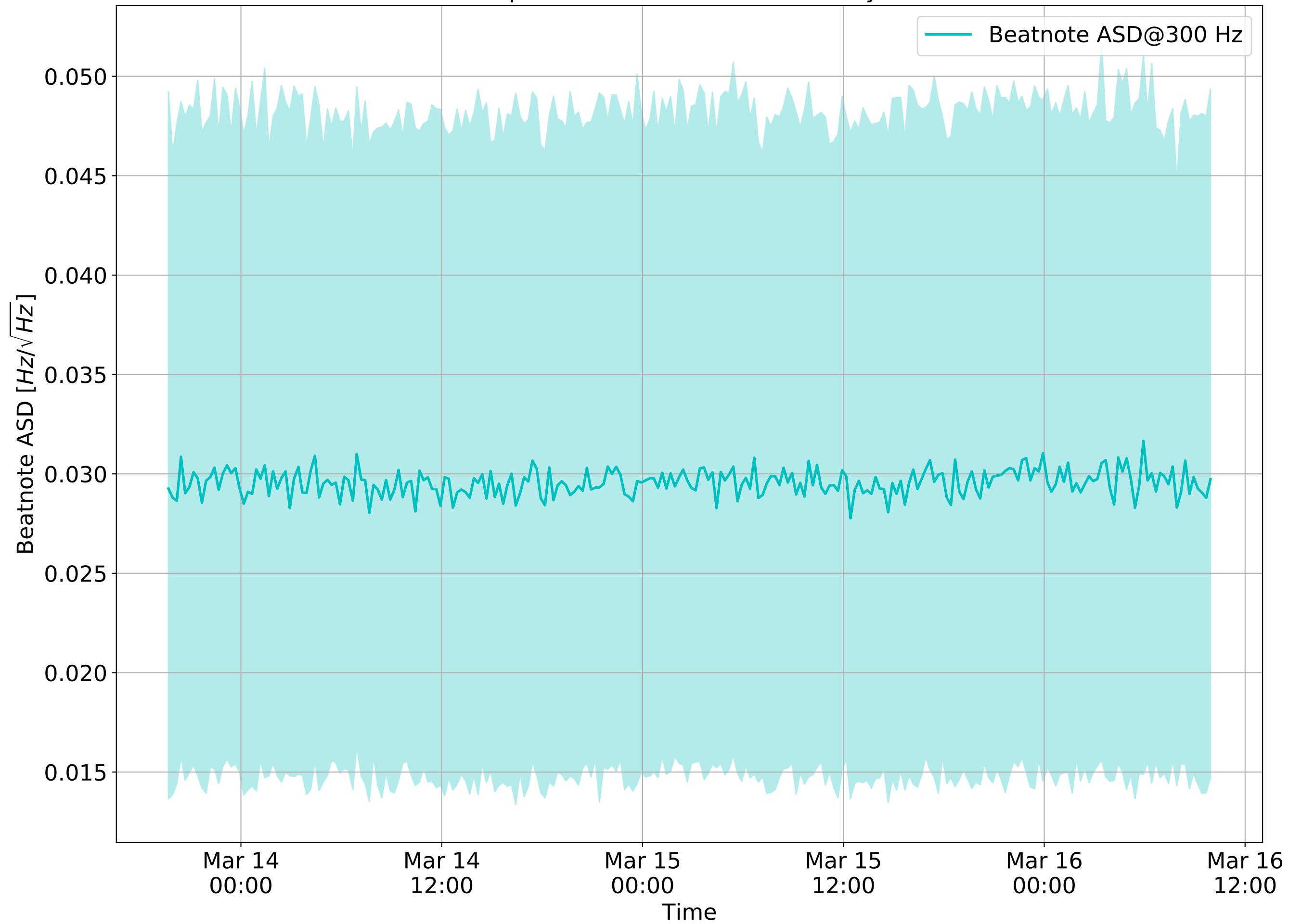
Beatnote Spectrum at different times of day at 300 Hz
