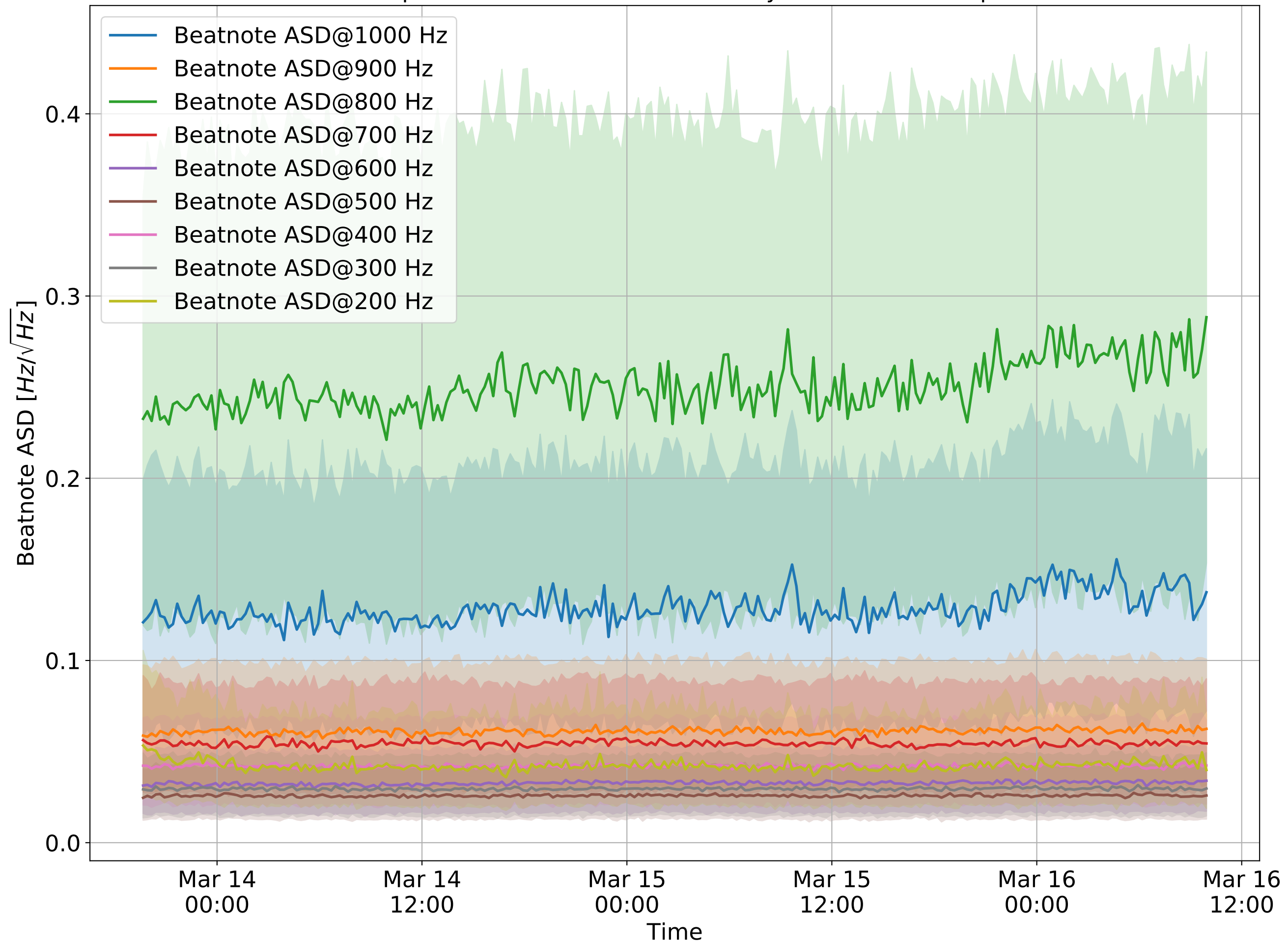
Beatnote Spectrum at different times of day and different frequencies
