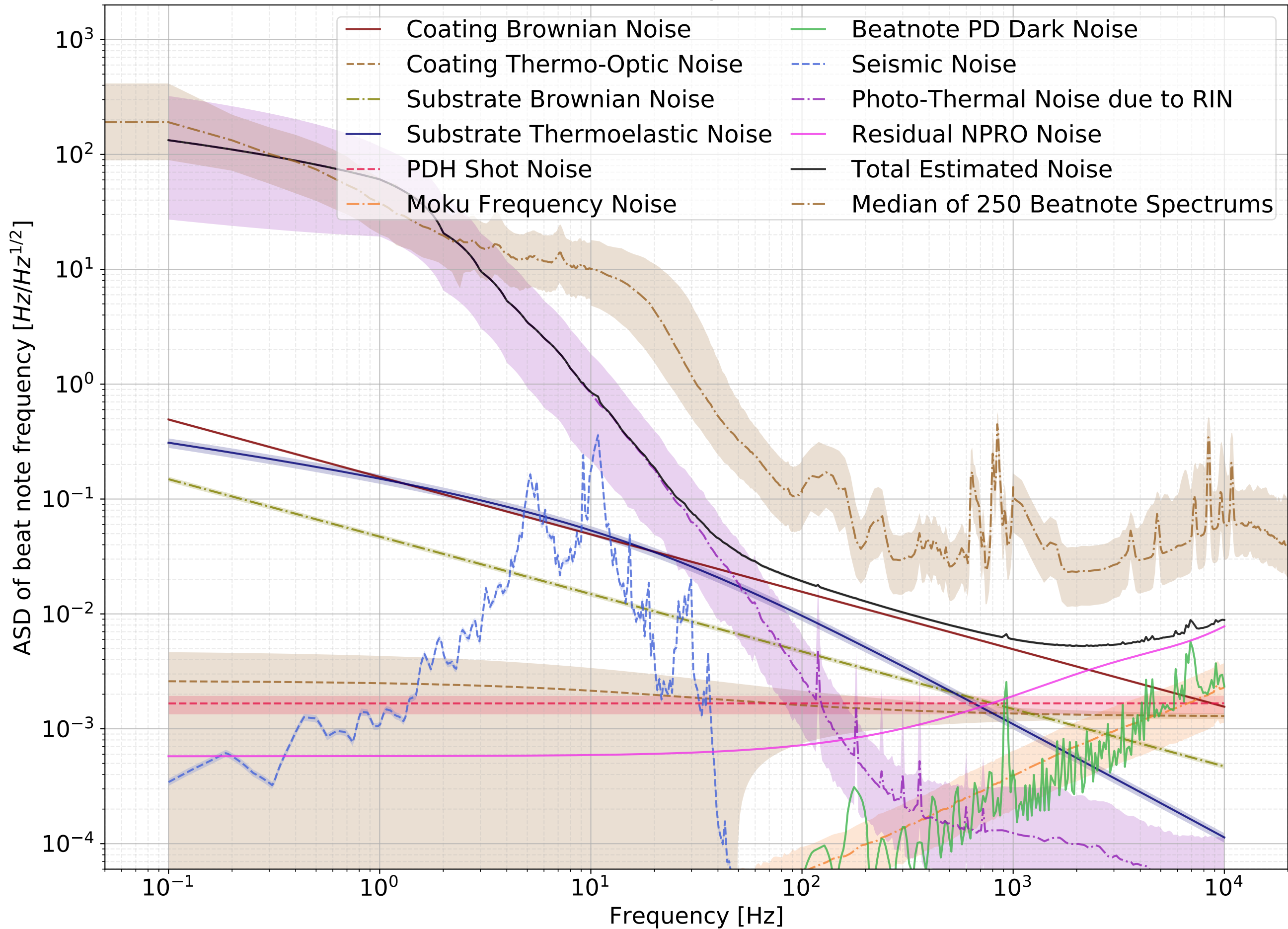
CTN Noise Budget, March 13-16, 2020 \Phi_B = (10 \pm 2) \times 10^{-5} ; \Phi_S = (2.1 \pm 2.1) \times 10^{-7}
