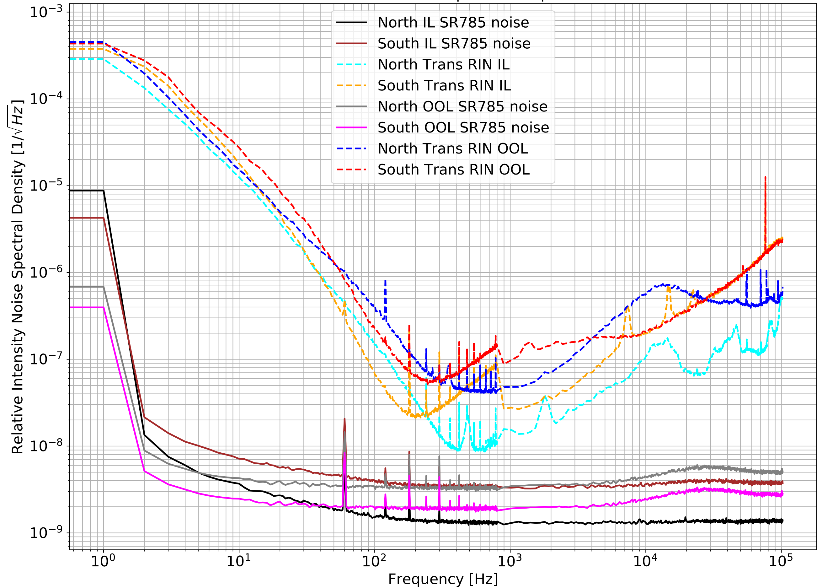
CTN Transmitted Laser RIN with ISS ON at G=20k OOL: Out-Of-Loop, IL: In-Loop
