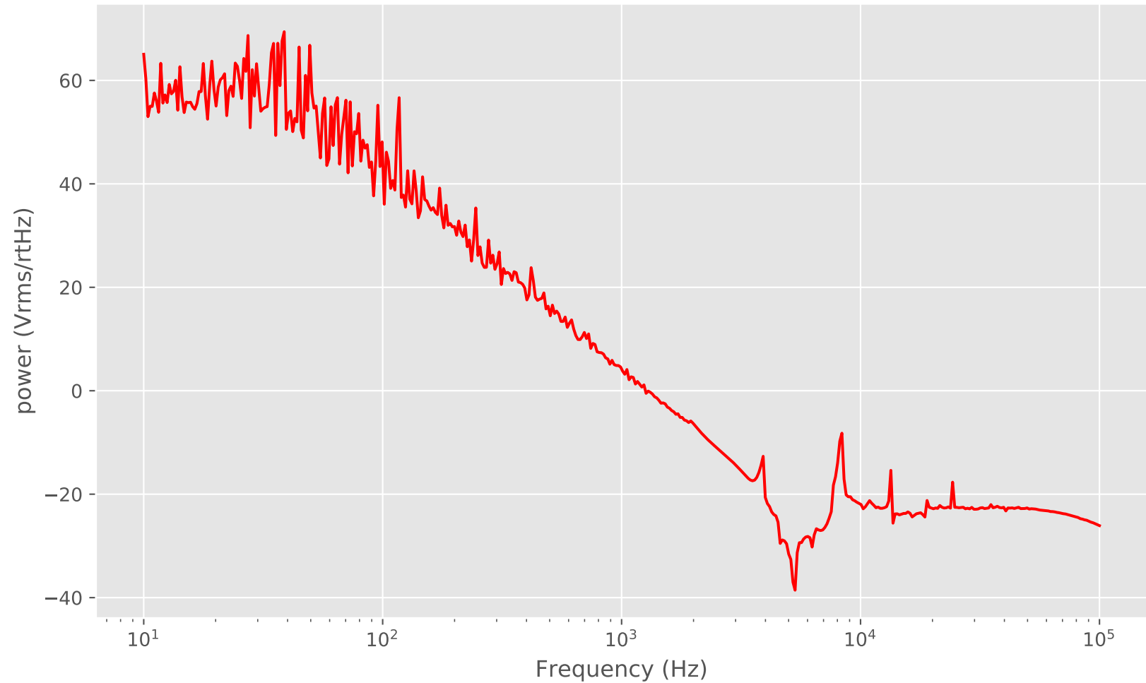
Plant Circuit TF Magnitude
