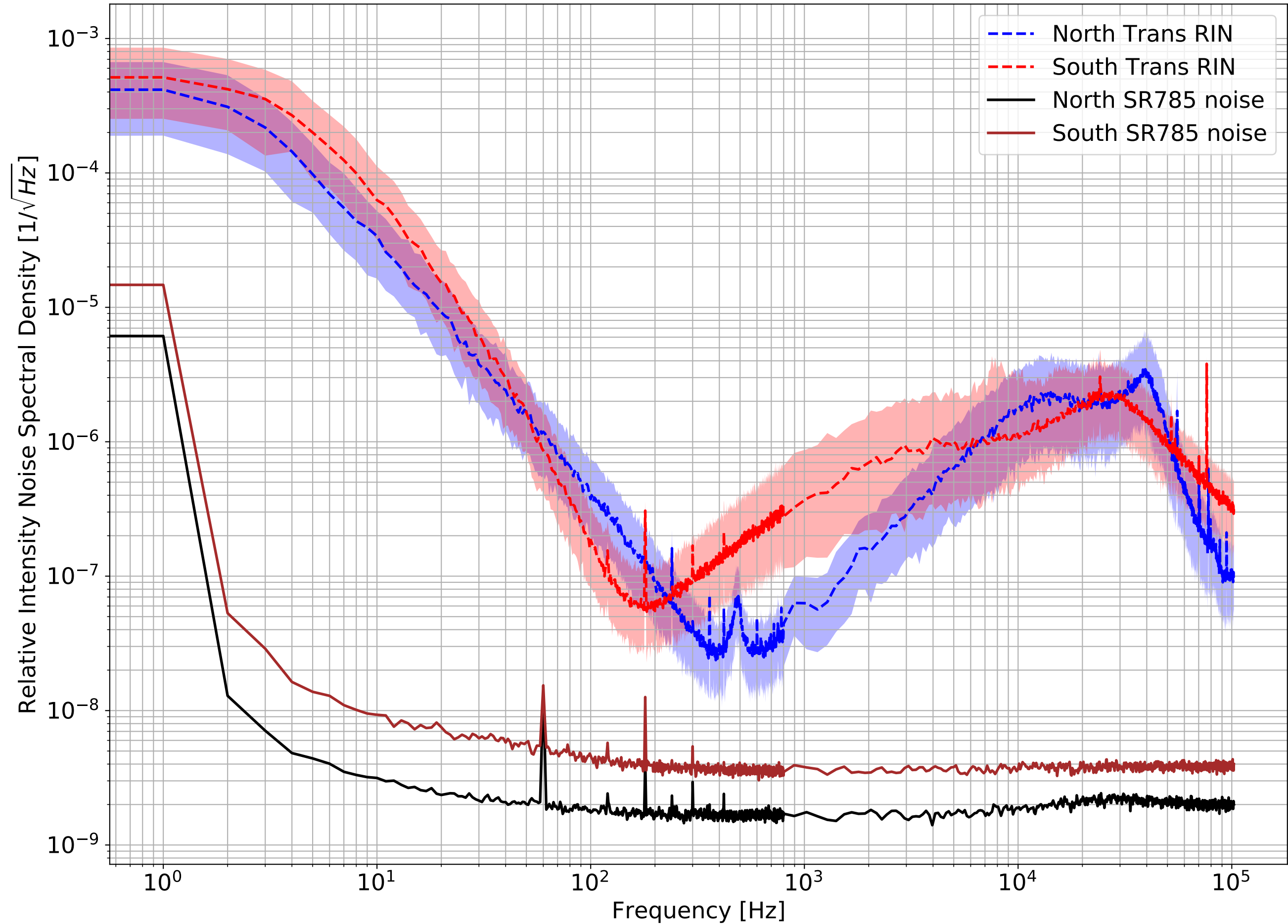
CTN Transmitted Laser RIN with ISS ON Median over 238 measurements. North Gain = 5000, South Gain = 5000
