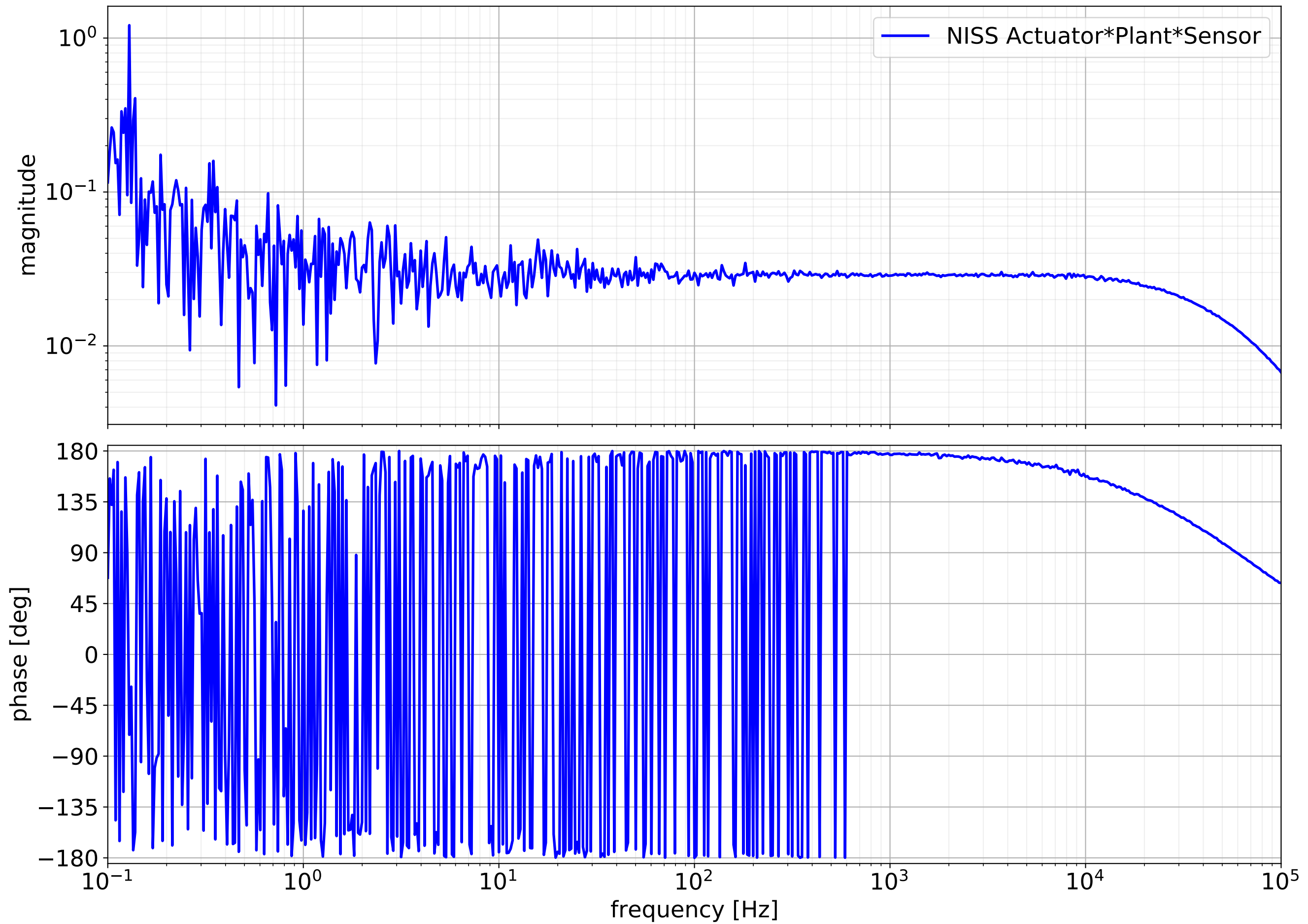
Measured Actuator-Plant-Sensor transfer function
