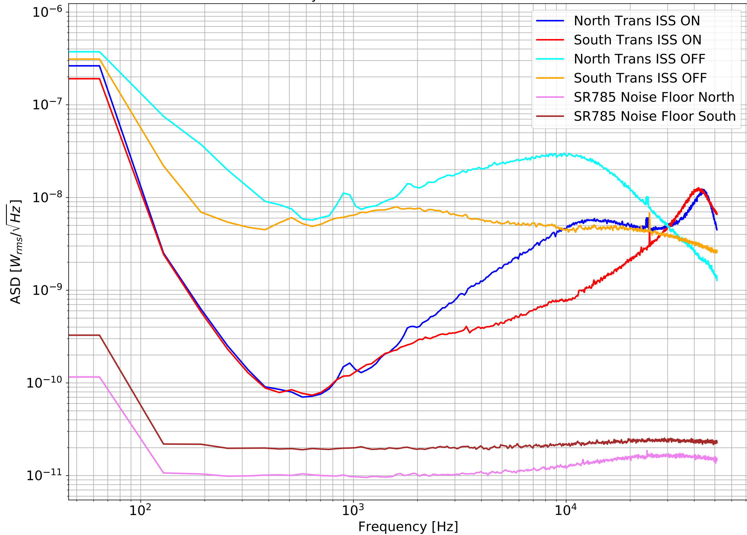
Intensity noise after transmission of Cavities
