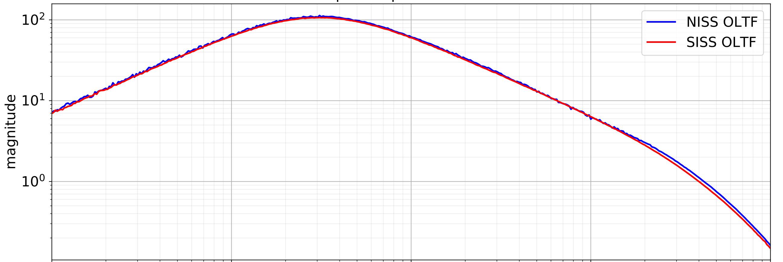
Measured Open Loop Transfer Function of ISS
