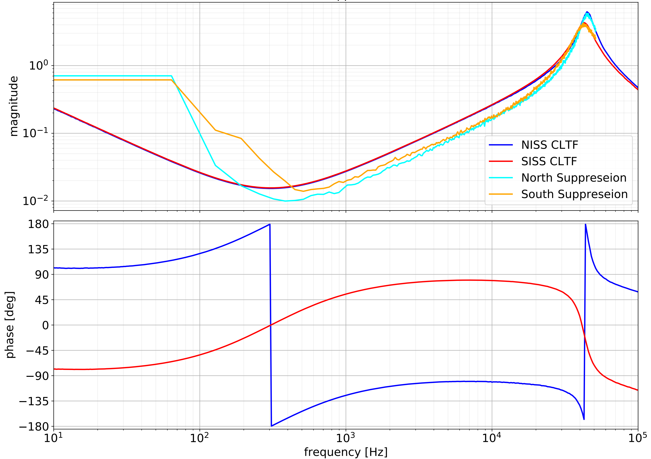
Measured Closed Loop Transfer Function of ISS v/s measured noise suppression at transmission
