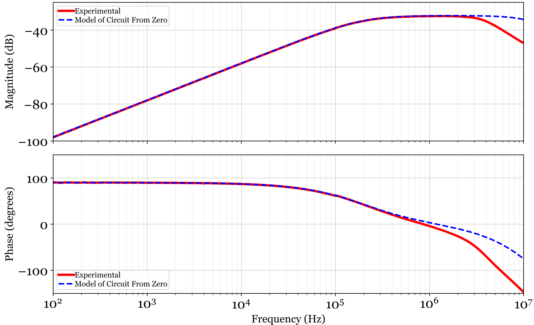
EOM Path Transfer Function
