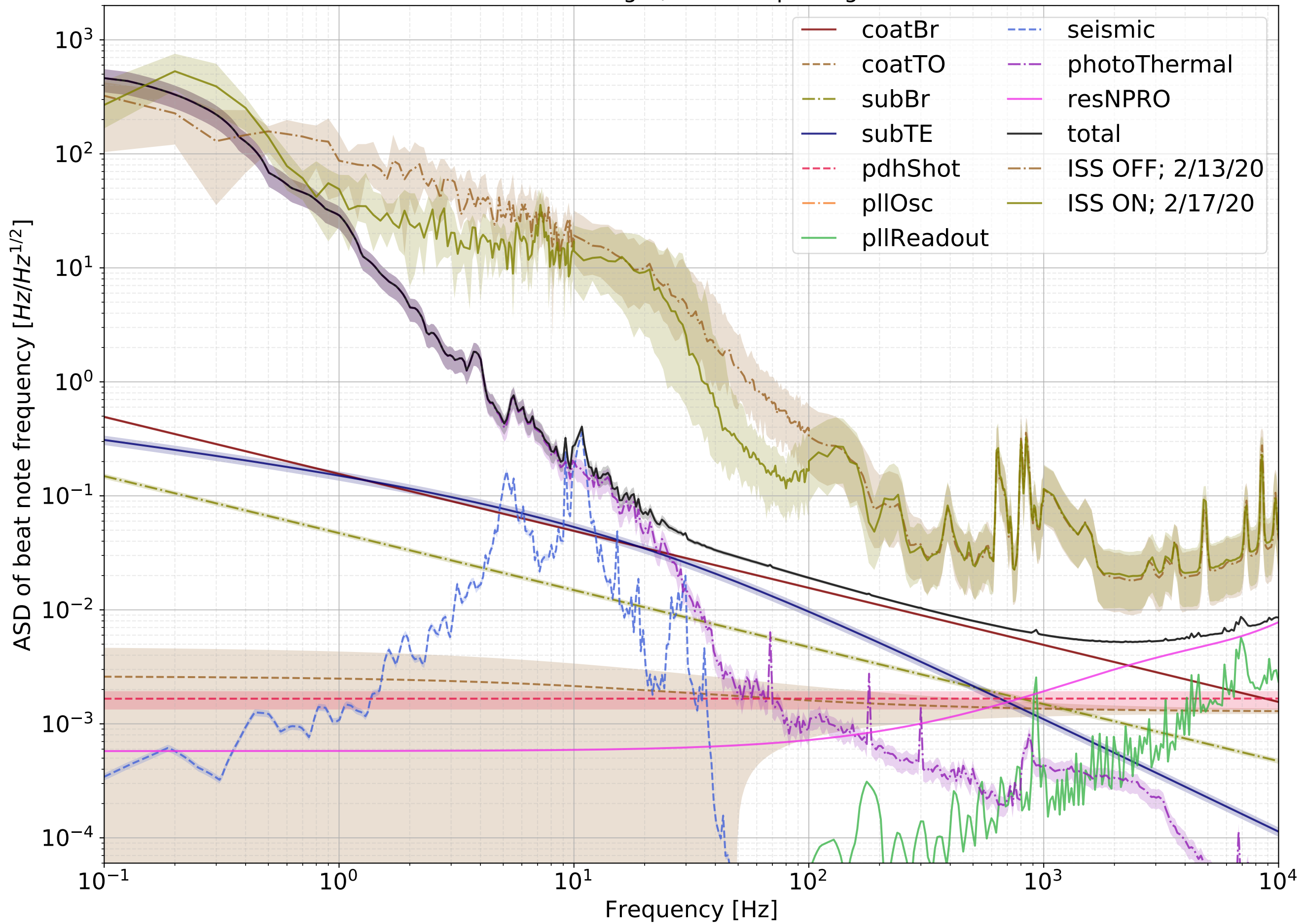
CTN Noise Budget, effect of putting in ISS
