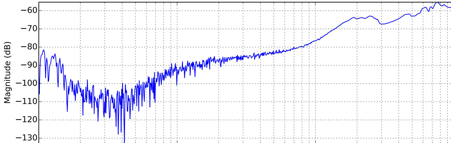
AG4395A TF Measurement For EOM Path - Feb 14 2020 - 16:58:03
