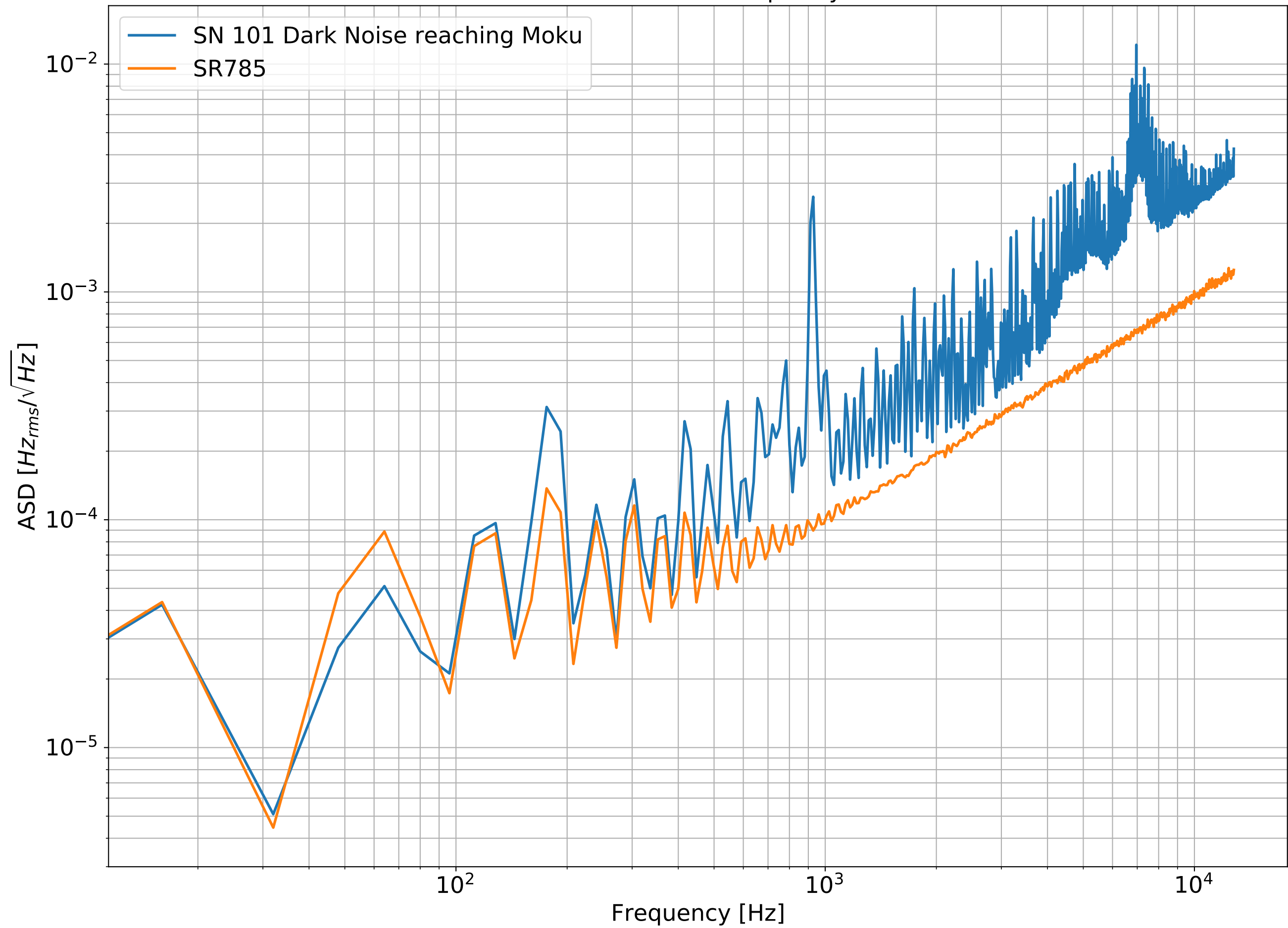
Dark Noise of Beatnote Detector SN 101 reaching Moku in terms of beatnote frequency noise
