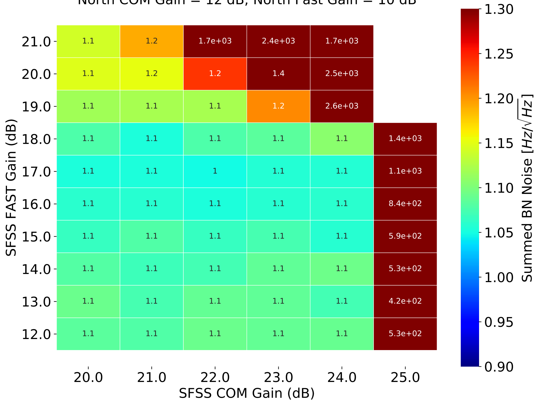
Beatnote frequency noise summed from 300 Hz to 600 Hz North COM Gain = 12 dB; North Fast Gain = 10 dB
