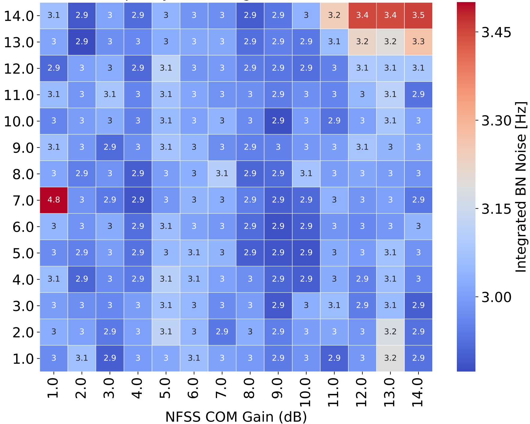
Beatnote frequency noise integrated from 200 Hz to 1 kHz
