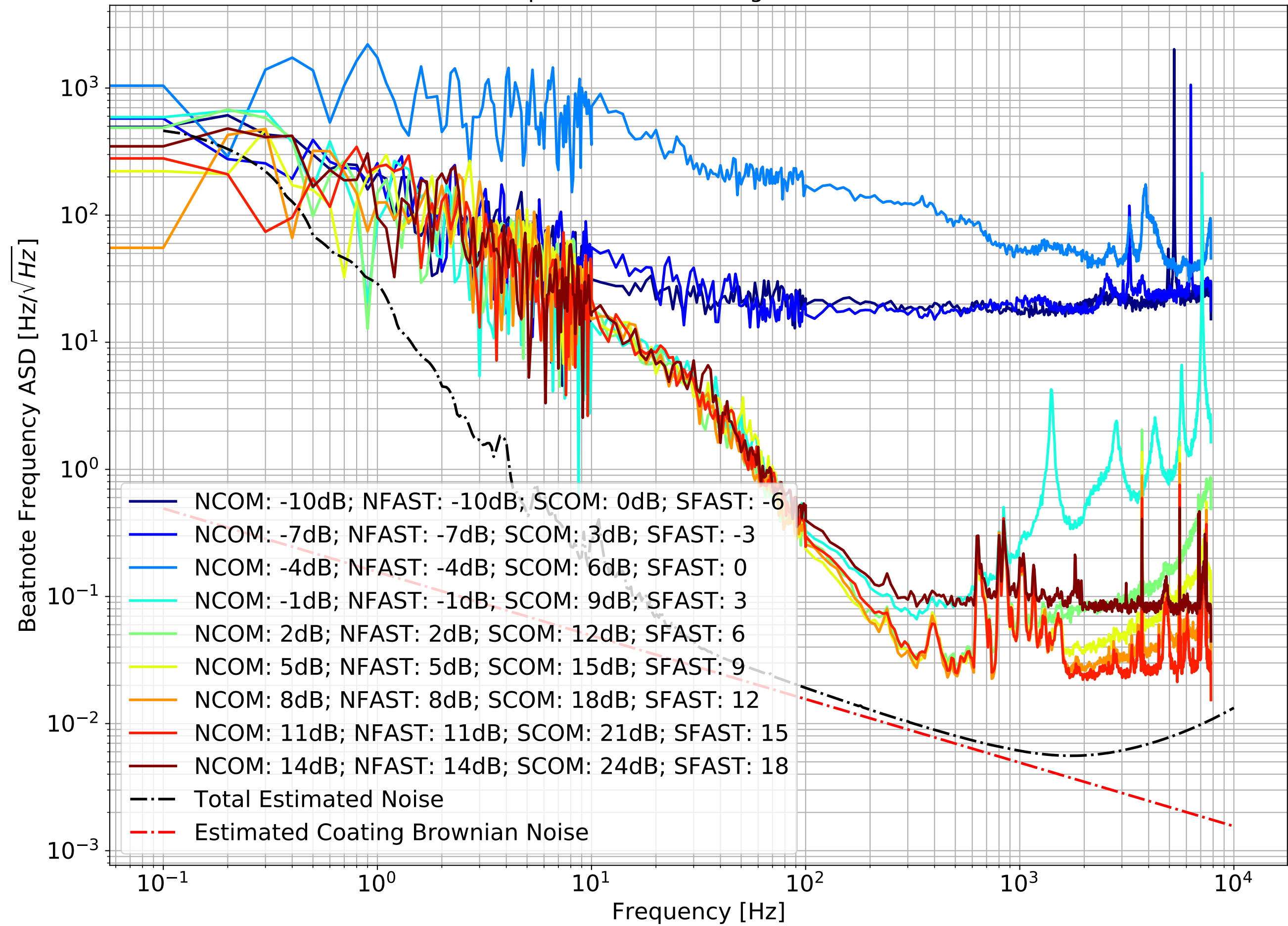
CTN Beatnote Spectrum when FSS gain values are increased.
