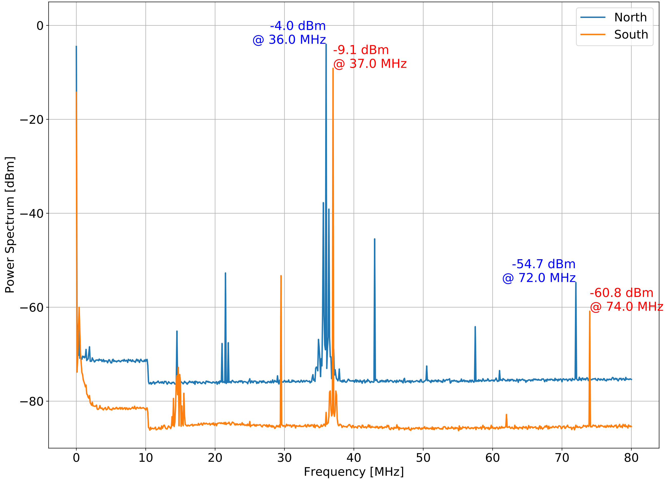
CTN FSS RFPD RF Out Spectrum when unlocked ResBW = 3 kHz
