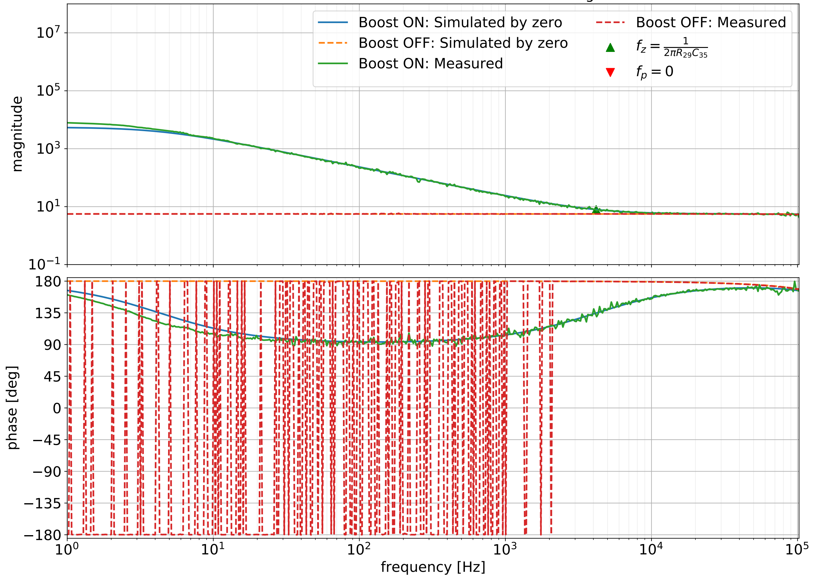
North FSS Box Transfer Function at Boost Stage
