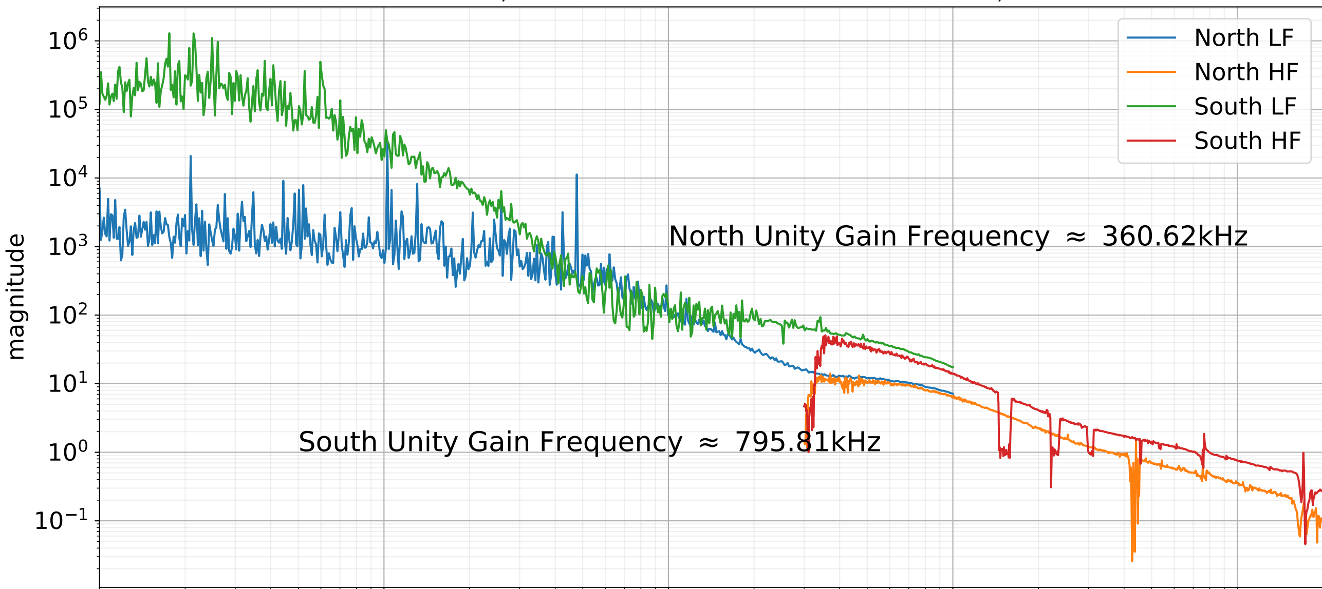
FSS Open Loop Gains - Boost On South: COMGain=24dB, FastGain=18dB North:COMGain=14dB, FASTGain=14dB
