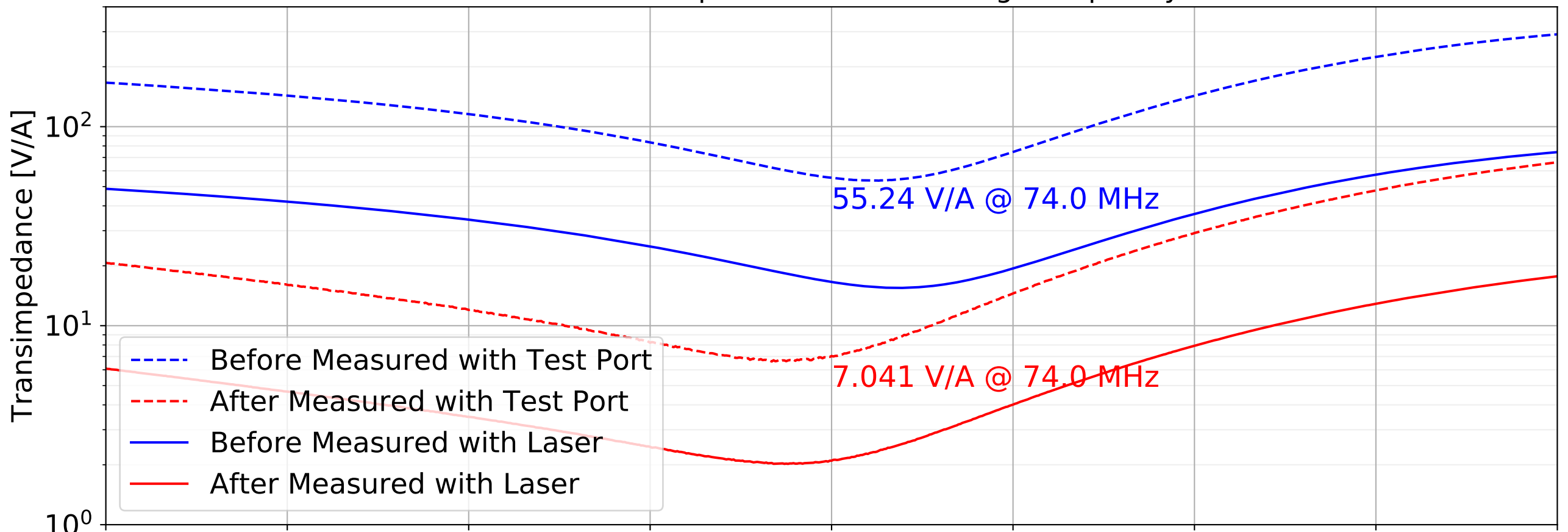
SN010 Transimpedance near 2-Omega frequency
