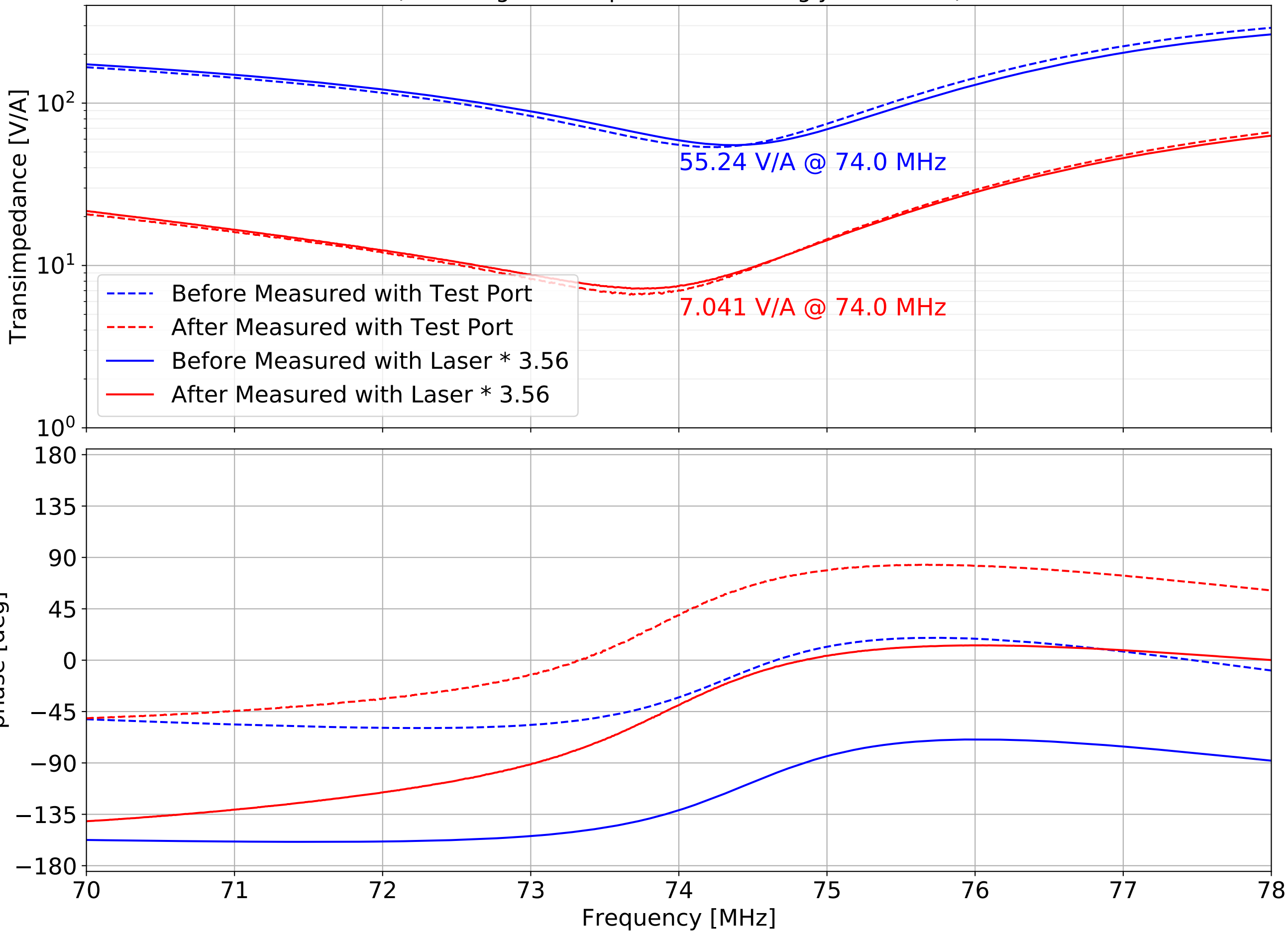
SN010 Transimpedance near 2-Omega frequency (Checking if DC impedance is wrongly estimated)
