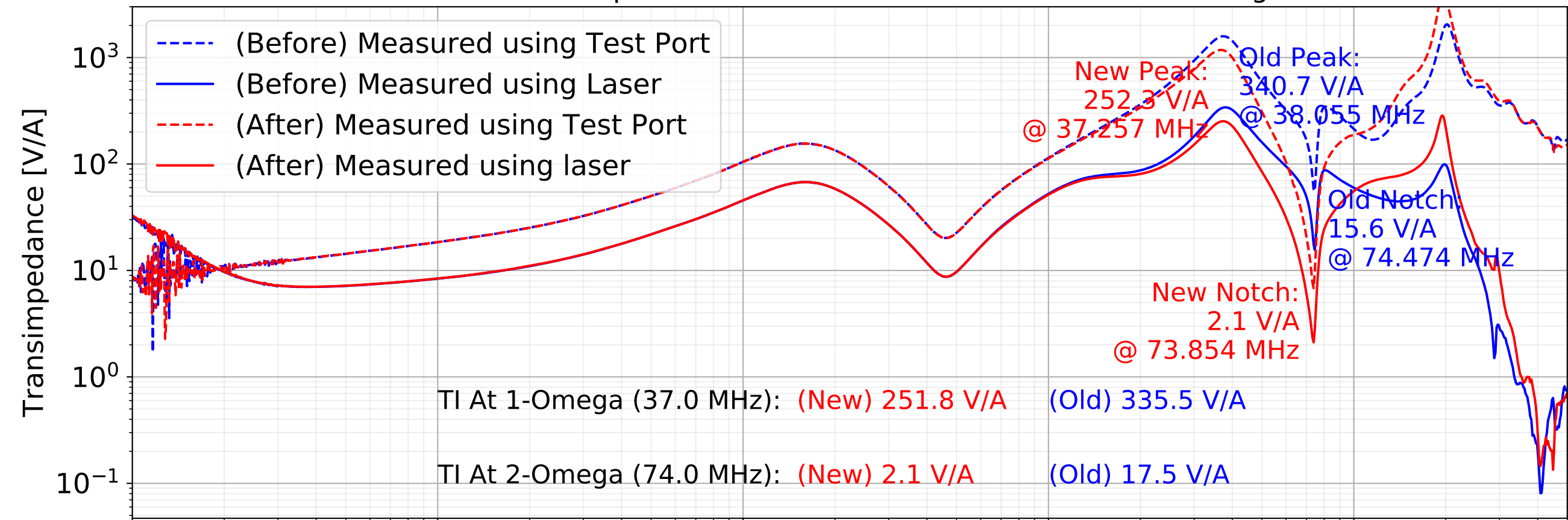
SN010 Transimpedance Measurement Before and After Changes
