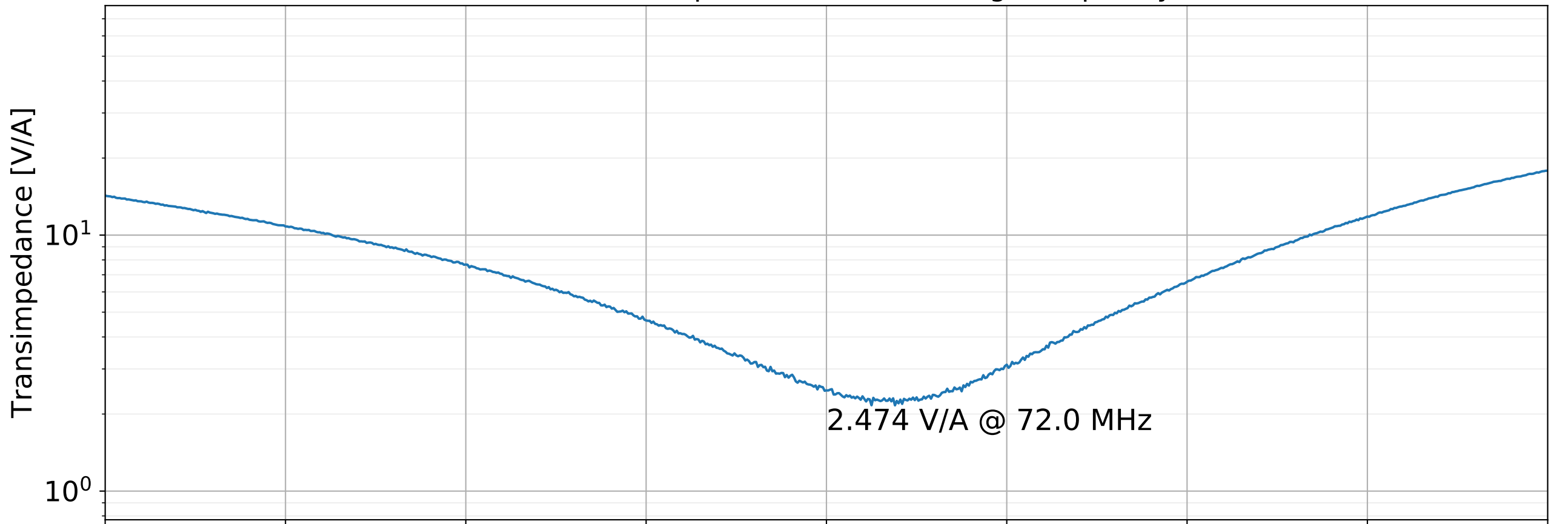
SN009 Transimpedance near 2-Omega frequency
