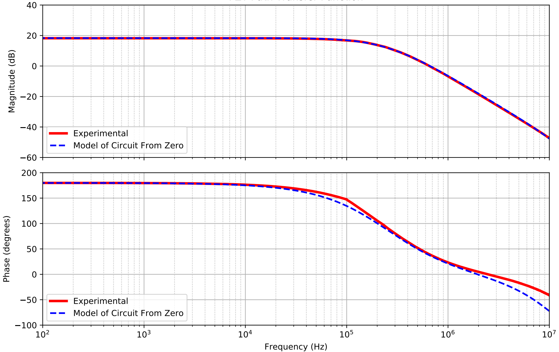
PZT Path Transfer Function
