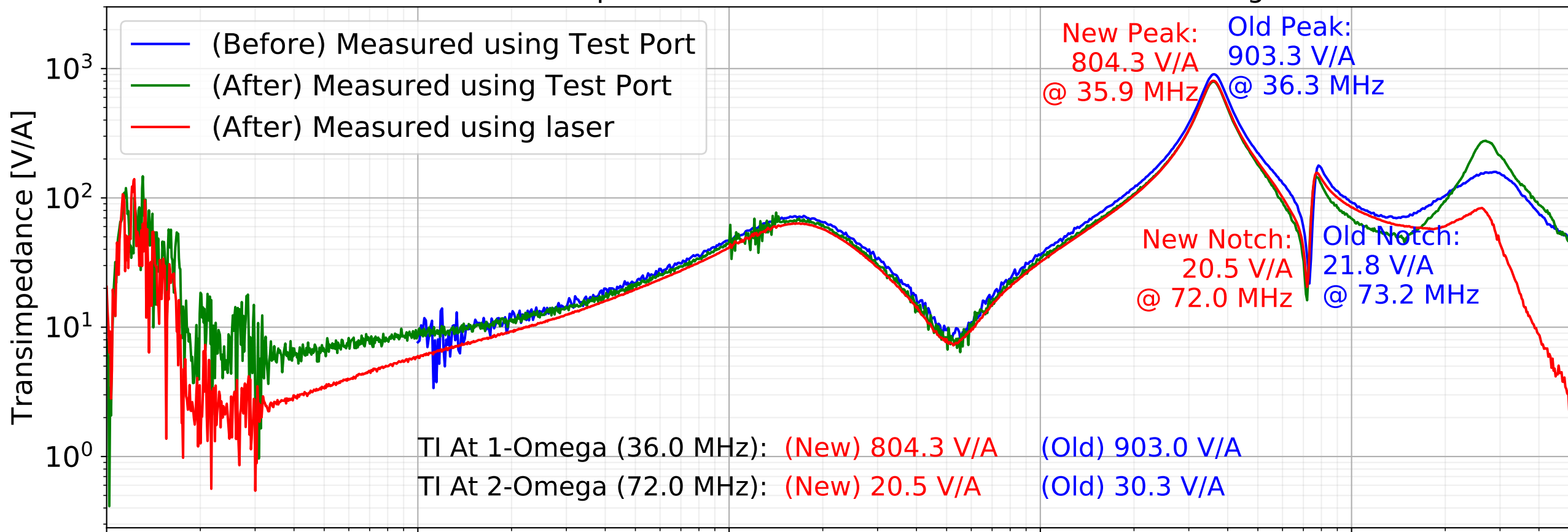
SN009 Transimpedance Measurement Before and After Changes
