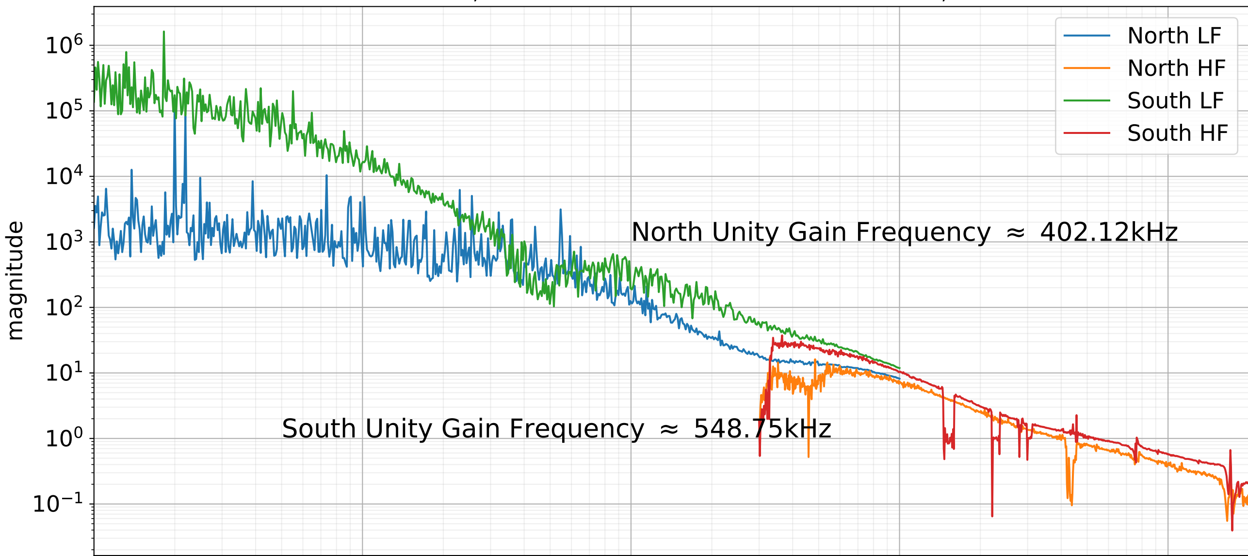
FSS Open Loop Gains - Boost On South: COMGain=24dB, FastGain=18dB North:COMGain=11dB, FASTGain=14dB
