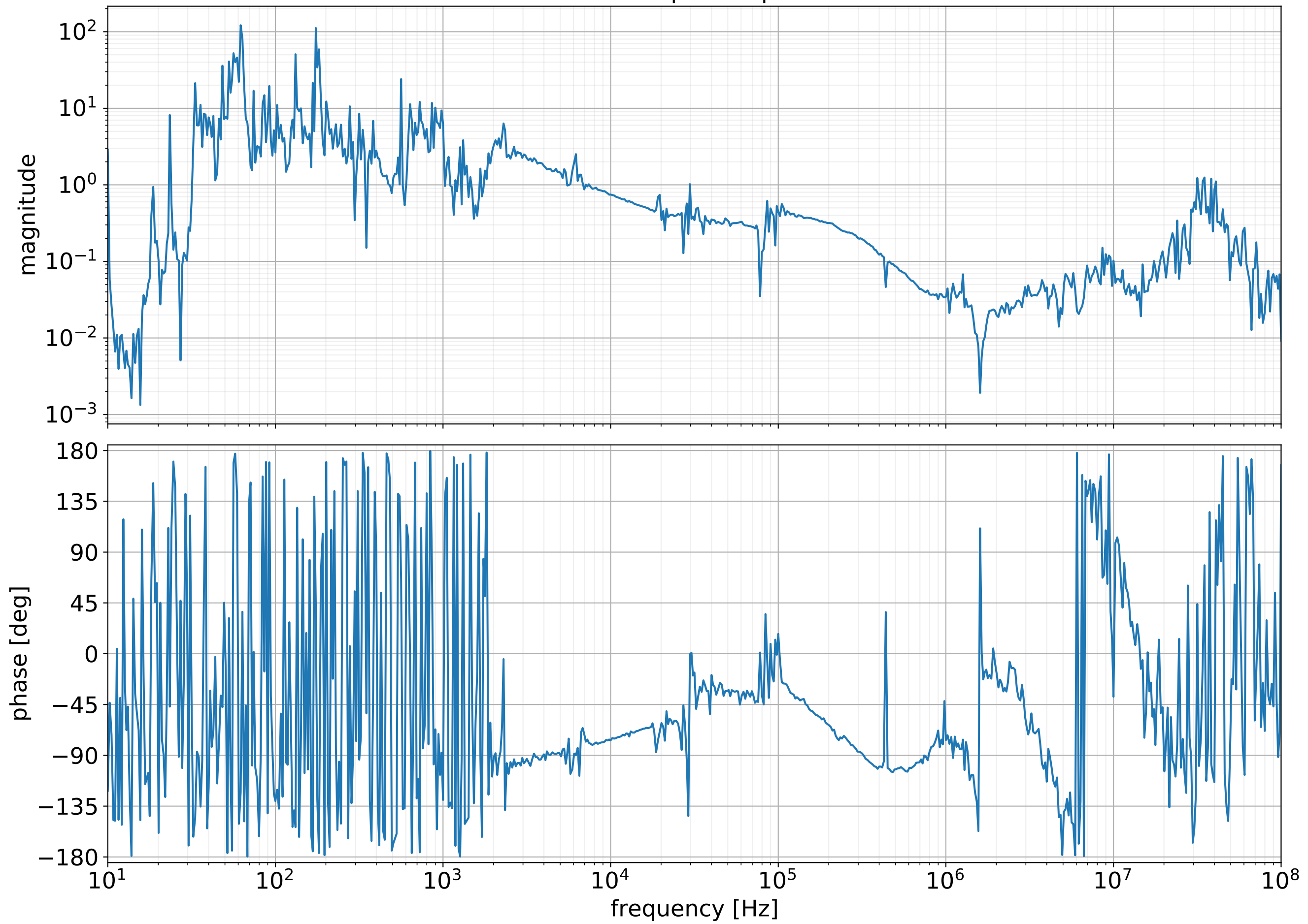
NPMC Open Loop TF
